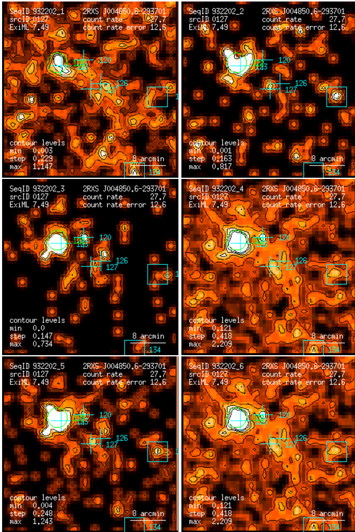
Figure 127: RASS 932202: detection 0127: band rate images, Gaussian filter: (1) PSPC channels 11 – 41, (2) 52 – 90, (3) 91 – 201, (4) 11 – 235, (5) 52 – 201, (6) 11 – 201. Broad band rates in counts/ks. Band rate contour levels in counts/ks/arcmin 2 .
