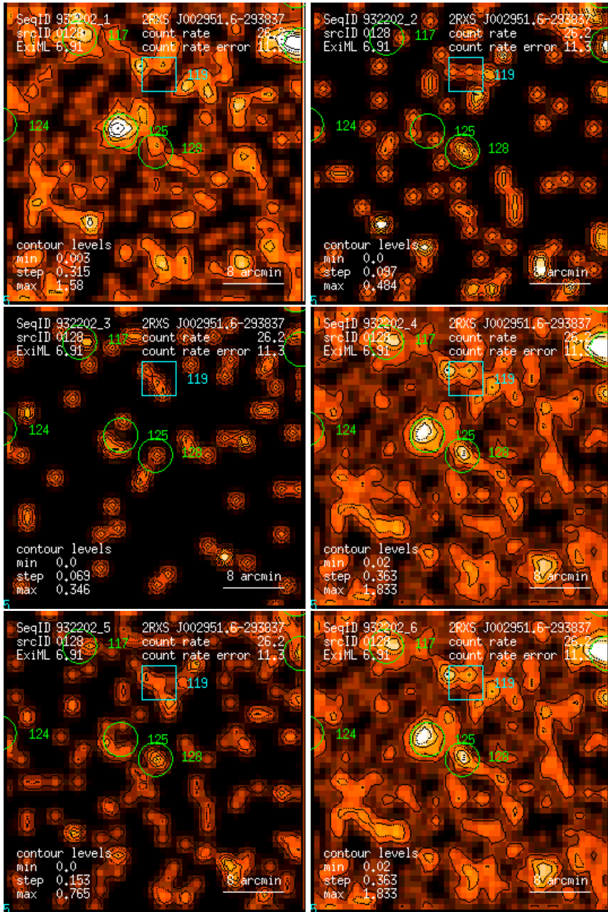
Figure 128: RASS 932202: detection 0128: band rate images, Gaussian filter: (1) PSPC channels 11 – 41, (2) 52 – 90, (3) 91 – 201, (4) 11 – 235, (5) 52 – 201, (6) 11 – 201. Broad band rates in counts/ks. Band rate contour levels in counts/ks/arcmin 2 .
