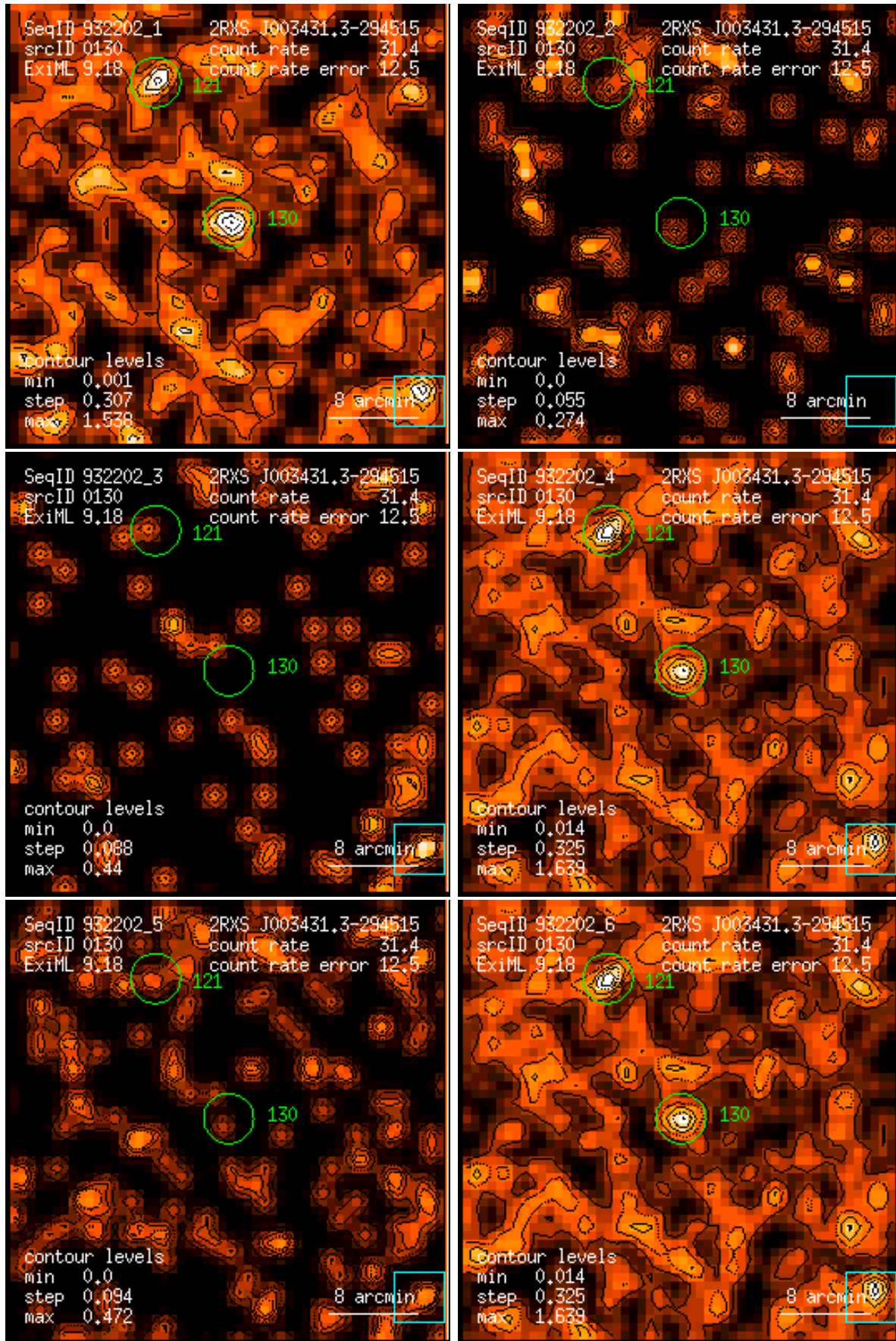
Figure 130: RASS 932202: detection 0130: band rate images, Gaussian filter: (1) PSPC channels 11 – 41, (2) 52 – 90, (3) 91 – 201, (4) 11 – 235, (5) 52 – 201, (6) 11 – 201. Broad band rates in counts/ks. Band rate contour levels in counts/ks/arcmin 2 .
