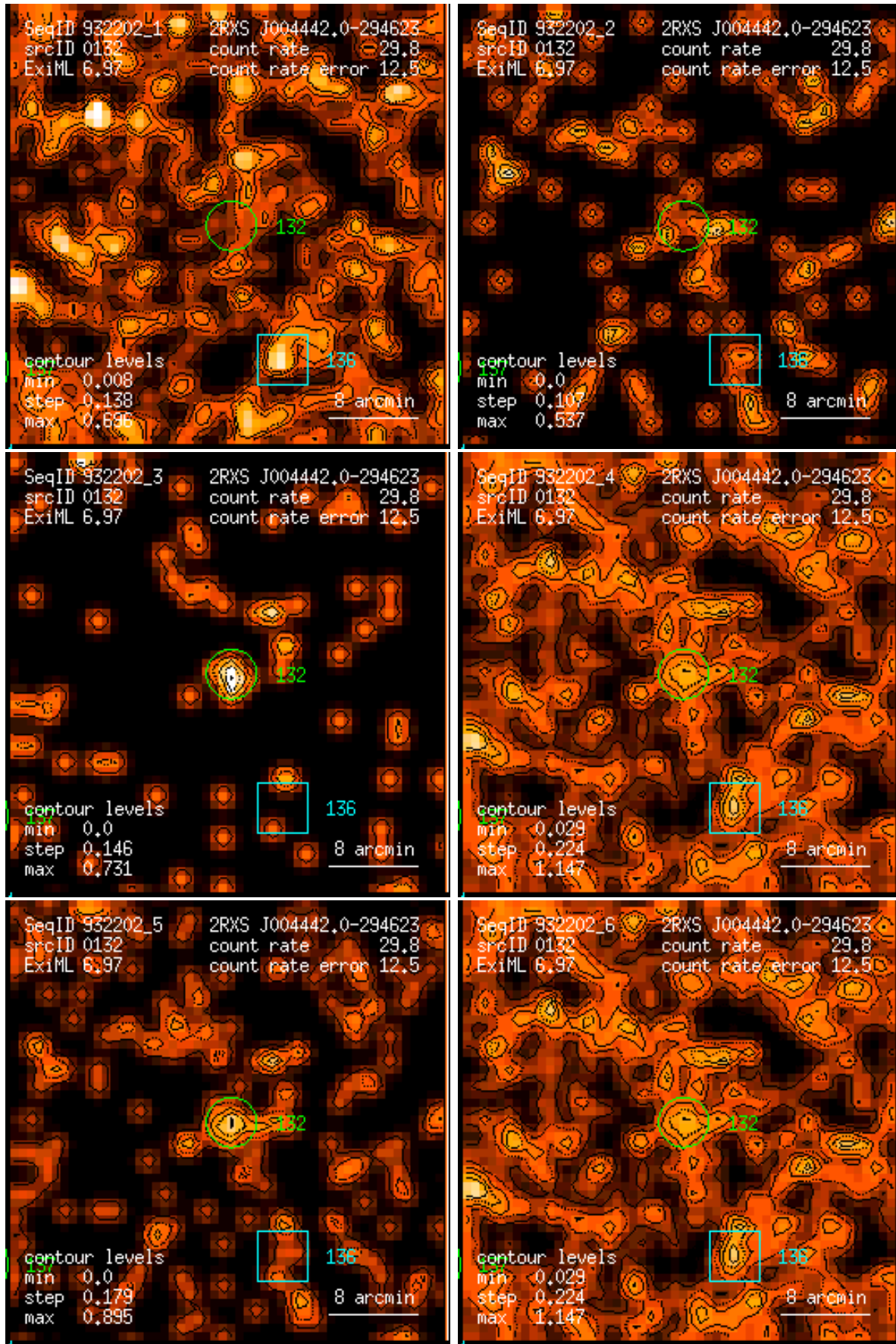
Figure 132: RASS 932202: detection 0132: band rate images, Gaussian filter: (1) PSPC channels 11 – 41, (2) 52 – 90, (3) 91 – 201, (4) 11 – 235, (5) 52 – 201, (6) 11 – 201. Broad band rates in counts/ks. Band rate contour levels in counts/ks/arcmin 2 .
