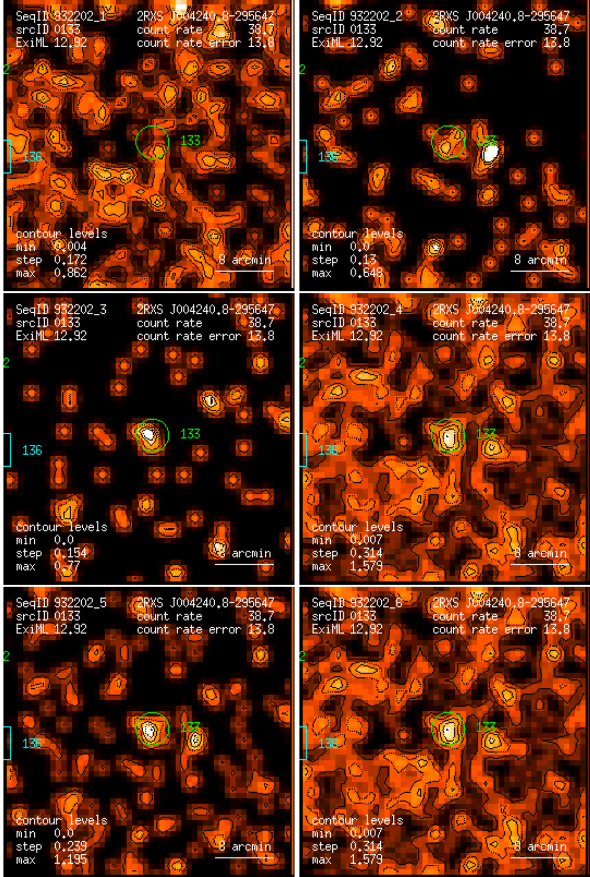
Figure 133: RASS 932202: detection 0133: band rate images, Gaussian filter: (1) PSPC channels 11 – 41, (2) 52 – 90, (3) 91 – 201, (4) 11 – 235, (5) 52 – 201, (6) 11 – 201. Broad band rates in counts/ks. Band rate contour levels in counts/ks/arcmin 2 .
