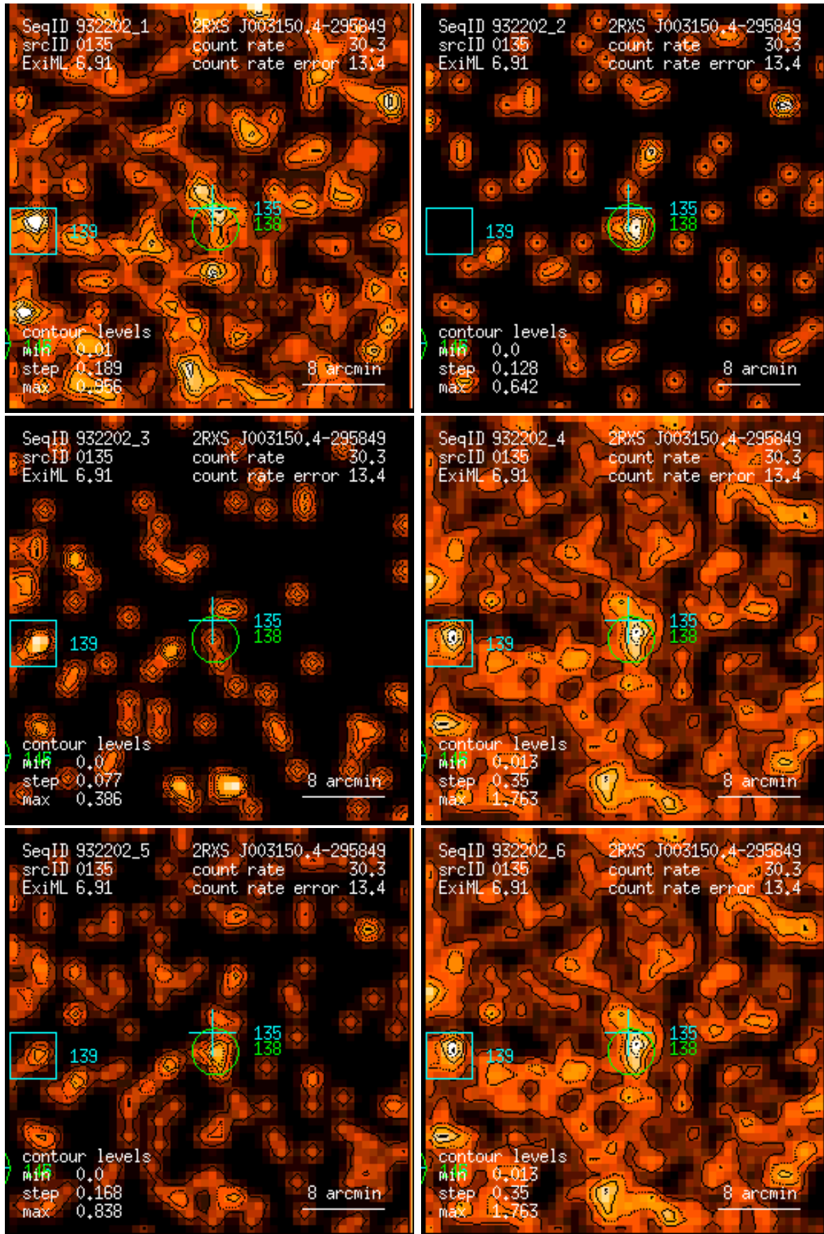
Figure 135: RASS 932202: detection 0135: band rate images, Gaussian filter: (1) PSPC channels 11 – 41, (2) 52 – 90, (3) 91 – 201, (4) 11 – 235, (5) 52 – 201, (6) 11 – 201. Broad band rates in counts/ks. Band rate contour levels in counts/ks/arcmin 2 .
