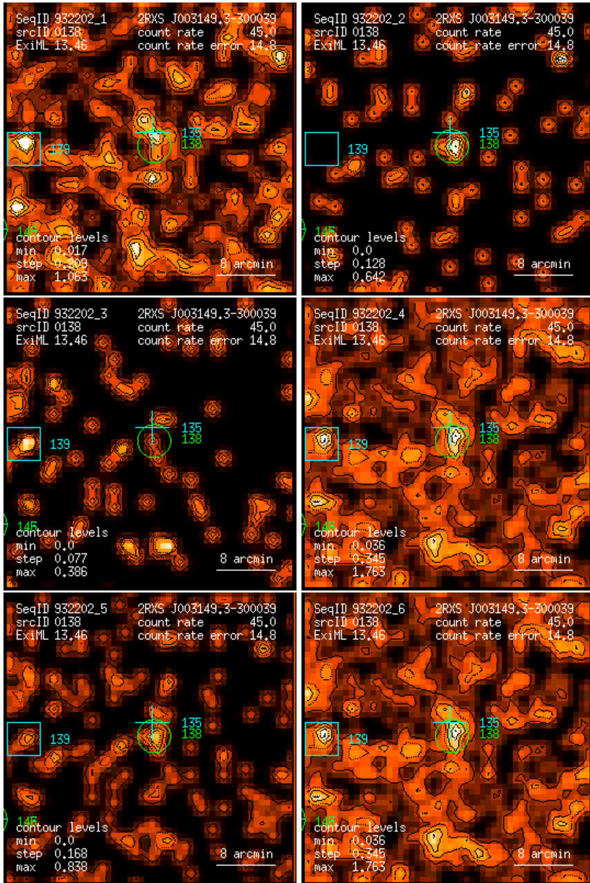
Figure 138: RASS 932202: detection 0138: band rate images, Gaussian filter: (1) PSPC channels 11 – 41, (2) 52 – 90, (3) 91 – 201, (4) 11 – 235, (5) 52 – 201, (6) 11 – 201. Broad band rates in counts/ks. Band rate contour levels in counts/ks/arcmin 2 .
