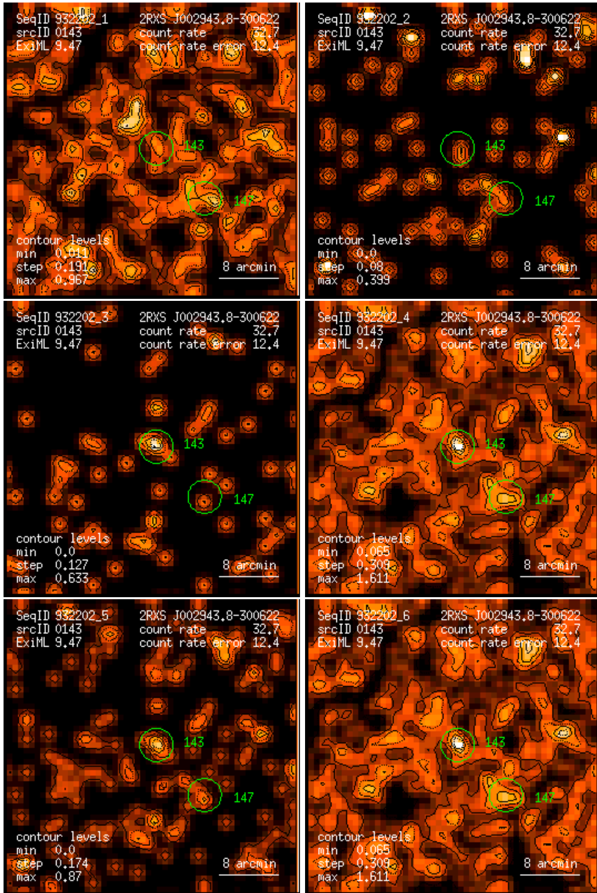
Figure 143: RASS 932202: detection 0143: band rate images, Gaussian filter: (1) PSPC channels 11 – 41, (2) 52 – 90, (3) 91 – 201, (4) 11 – 235, (5) 52 – 201, (6) 11 – 201. Broad band rates in counts/ks. Band rate contour levels in counts/ks/arcmin 2 .
