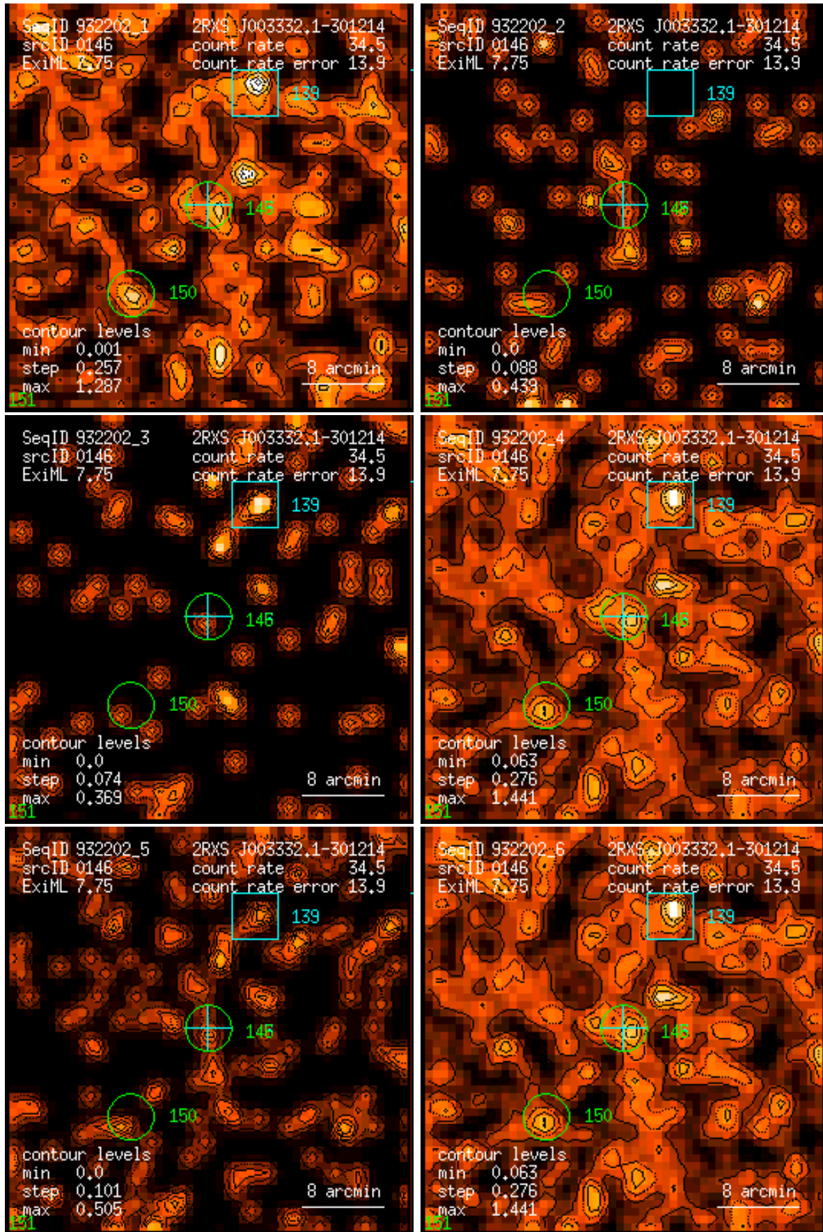
Figure 146: RASS 932202: detection 0146: band rate images, Gaussian filter: (1) PSPC channels 11 – 41, (2) 52 – 90, (3) 91 – 201, (4) 11 – 235, (5) 52 – 201, (6) 11 – 201. Broad band rates in counts/ks. Band rate contour levels in counts/ks/arcmin 2 .
