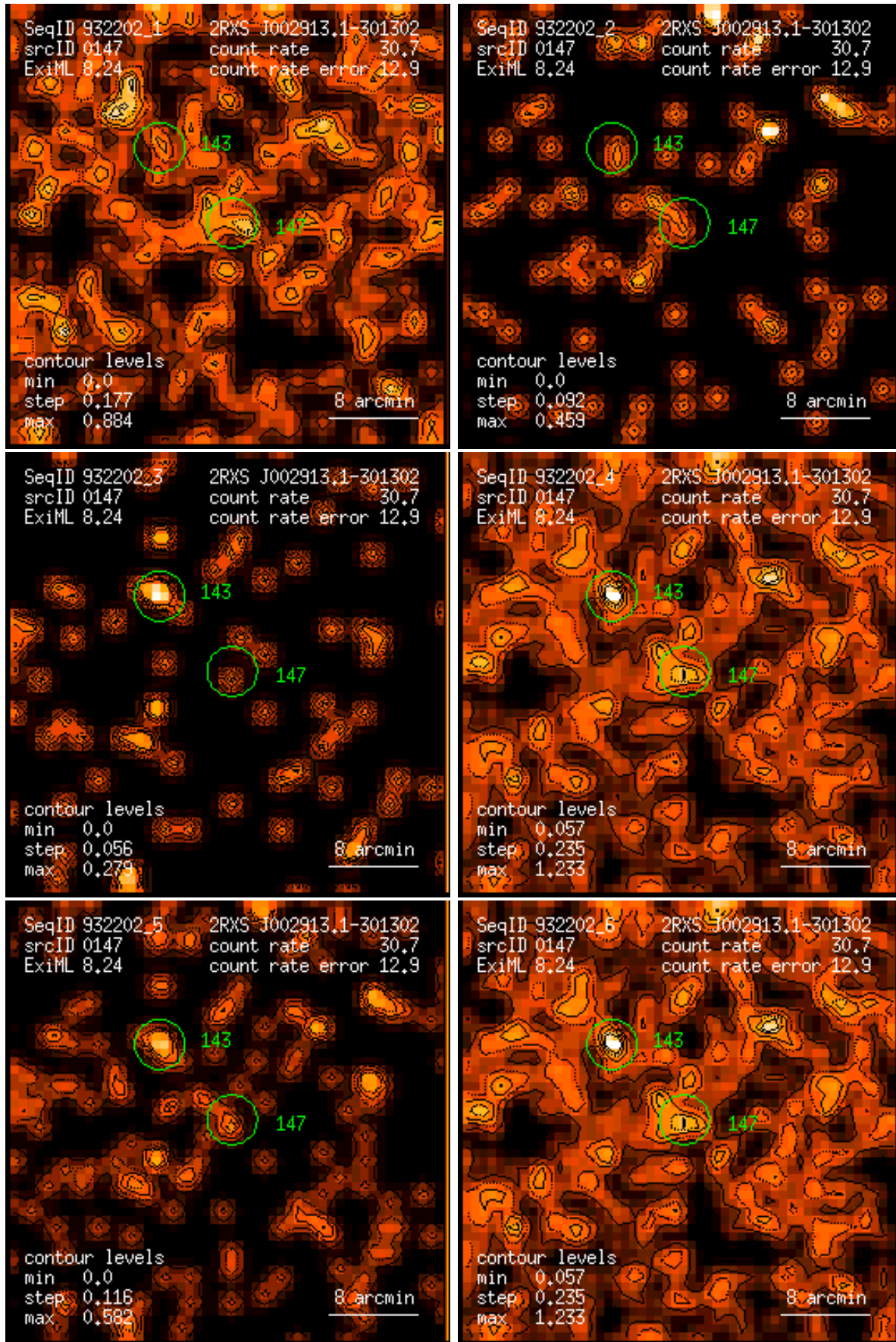
Figure 147: RASS 932202: detection 0147: band rate images, Gaussian filter: (1) PSPC channels 11 – 41, (2) 52 – 90, (3) 91 – 201, (4) 11 – 235, (5) 52 – 201, (6) 11 – 201. Broad band rates in counts/ks. Band rate contour levels in counts/ks/arcmin 2 .
