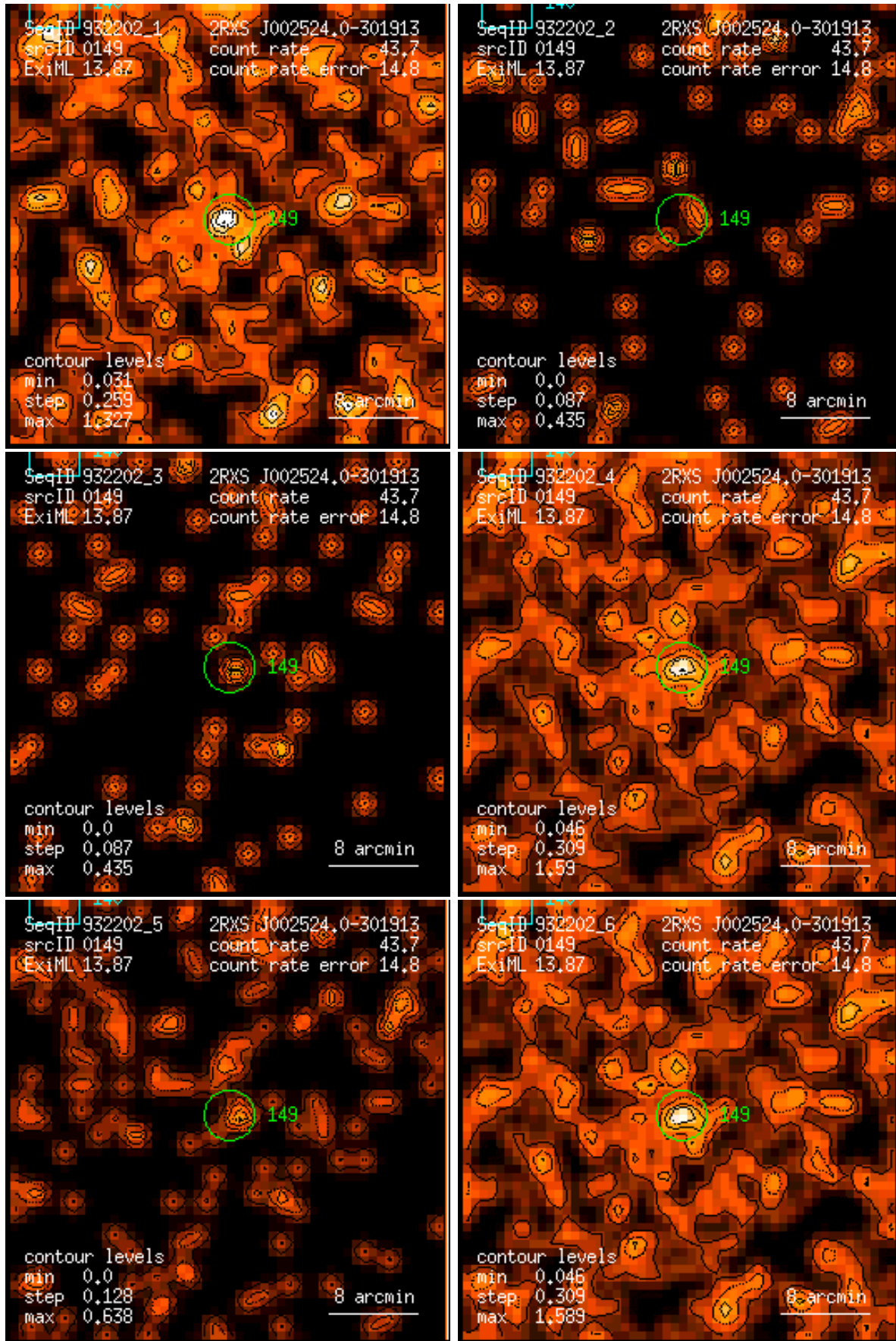
Figure 149: RASS 932202: detection 0149: band rate images, Gaussian filter: (1) PSPC channels 11 – 41, (2) 52 – 90, (3) 91 – 201, (4) 11 – 235, (5) 52 – 201, (6) 11 – 201. Broad band rates in counts/ks. Band rate contour levels in counts/ks/arcmin 2 .
