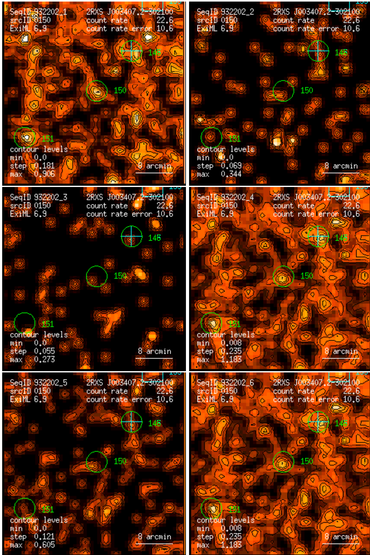
Figure 150: RASS 932202: detection 0150: band rate images, Gaussian filter: (1) PSPC channels 11 – 41, (2) 52 – 90, (3) 91 – 201, (4) 11 – 235, (5) 52 – 201, (6) 11 – 201. Broad band rates in counts/ks. Band rate contour levels in counts/ks/arcmin 2 .
