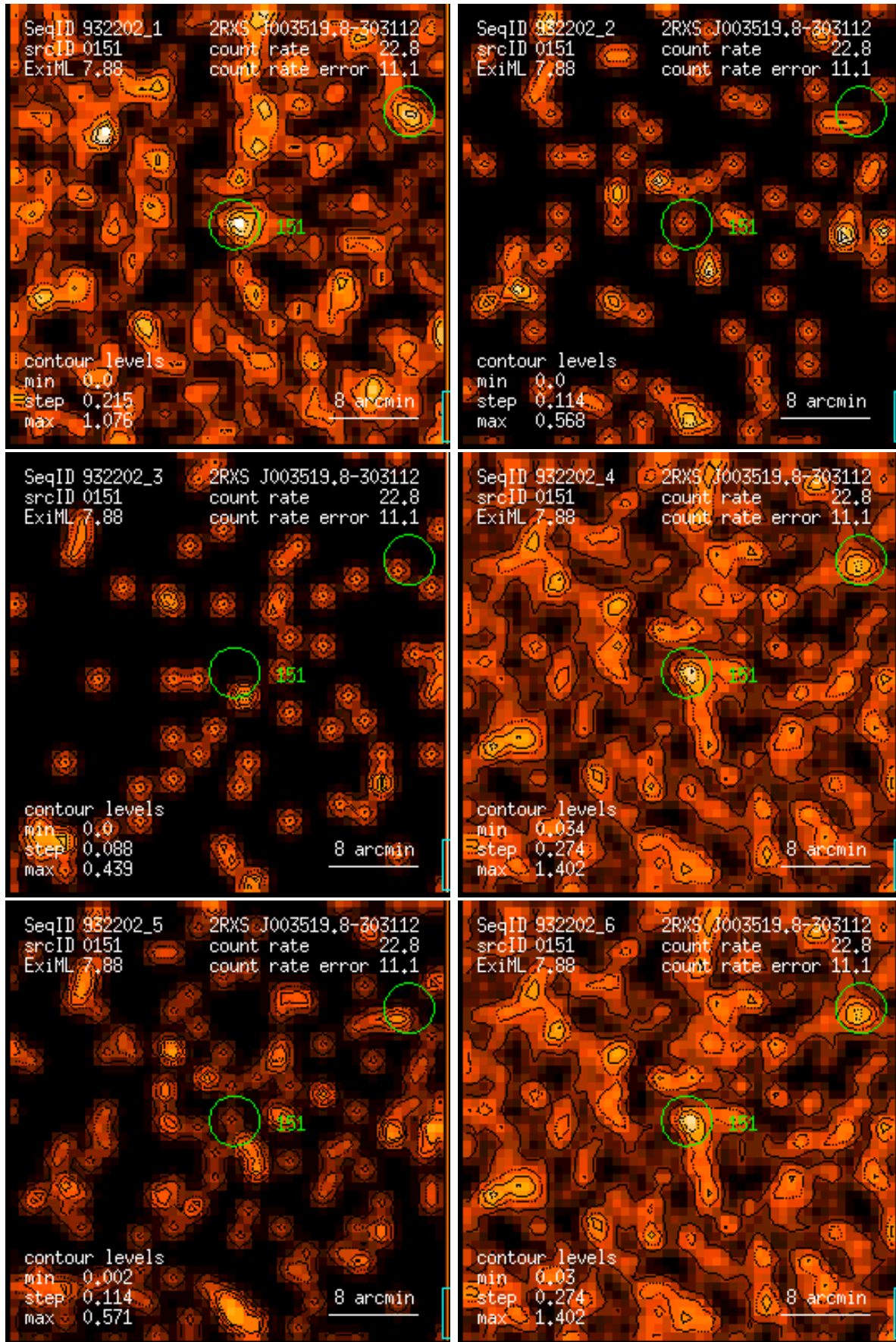
Figure 151: RASS 932202: detection 0151: band rate images, Gaussian filter: (1) PSPC channels 11 – 41, (2) 52 – 90, (3) 91 – 201, (4) 11 – 235, (5) 52 – 201, (6) 11 – 201. Broad band rates in counts/ks. Band rate contour levels in counts/ks/arcmin 2 .
