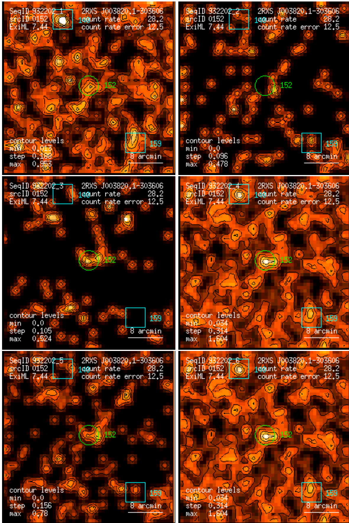
Figure 152: RASS 932202: detection 0152: band rate images, Gaussian filter: (1) PSPC channels 11 – 41, (2) 52 – 90, (3) 91 – 201, (4) 11 – 235, (5) 52 – 201, (6) 11 – 201. Broad band rates in counts/ks. Band rate contour levels in counts/ks/arcmin 2 .
