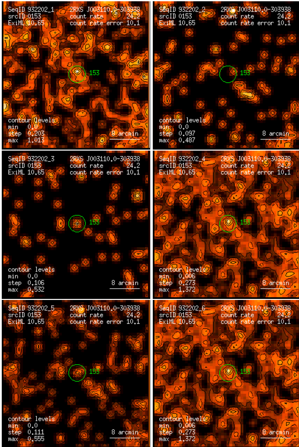
Figure 153: RASS 932202: detection 0153: band rate images, Gaussian filter: (1) PSPC channels 11 – 41, (2) 52 – 90, (3) 91 – 201, (4) 11 – 235, (5) 52 – 201, (6) 11 – 201. Broad band rates in counts/ks. Band rate contour levels in counts/ks/arcmin 2 .
