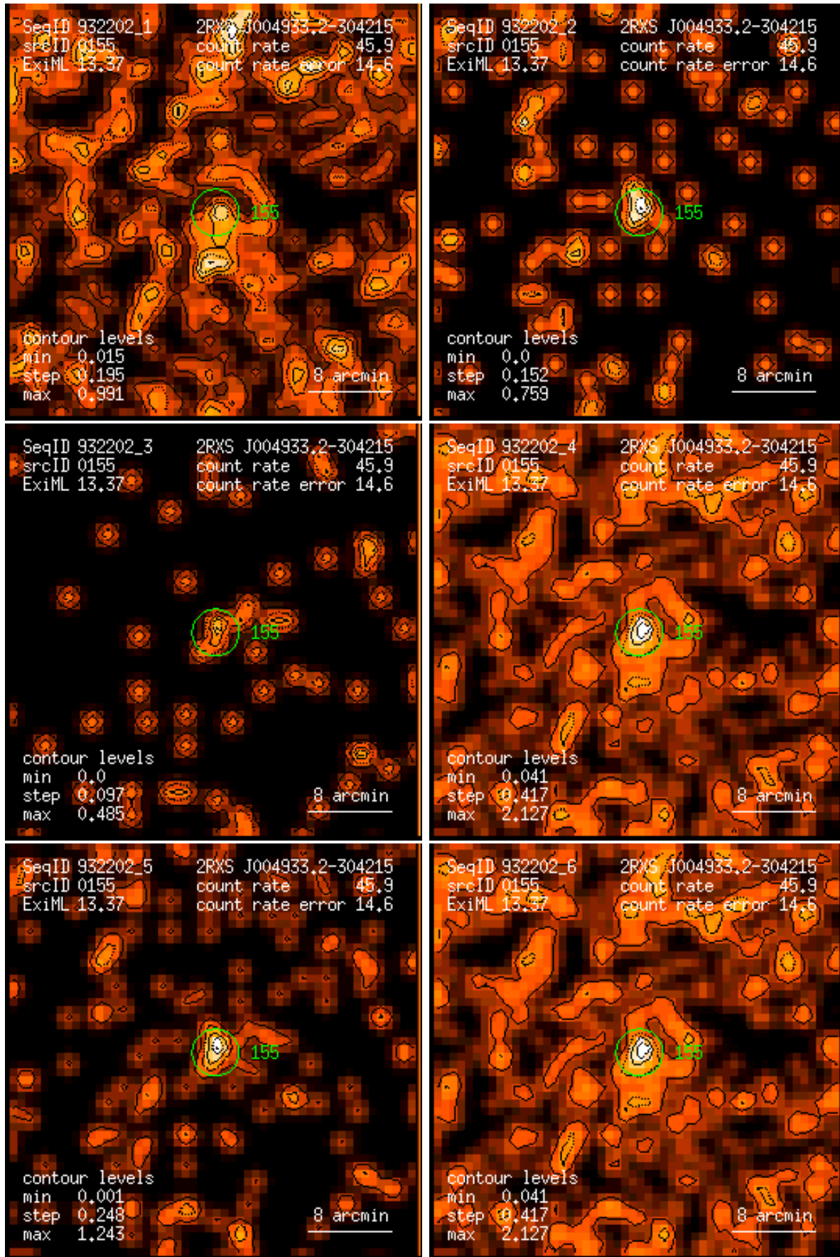
Figure 155: RASS 932202: detection 0155: band rate images, Gaussian filter: (1) PSPC channels 11 – 41, (2) 52 – 90, (3) 91 – 201, (4) 11 – 235, (5) 52 – 201, (6) 11 – 201. Broad band rates in counts/ks. Band rate contour levels in counts/ks/arcmin 2 .
