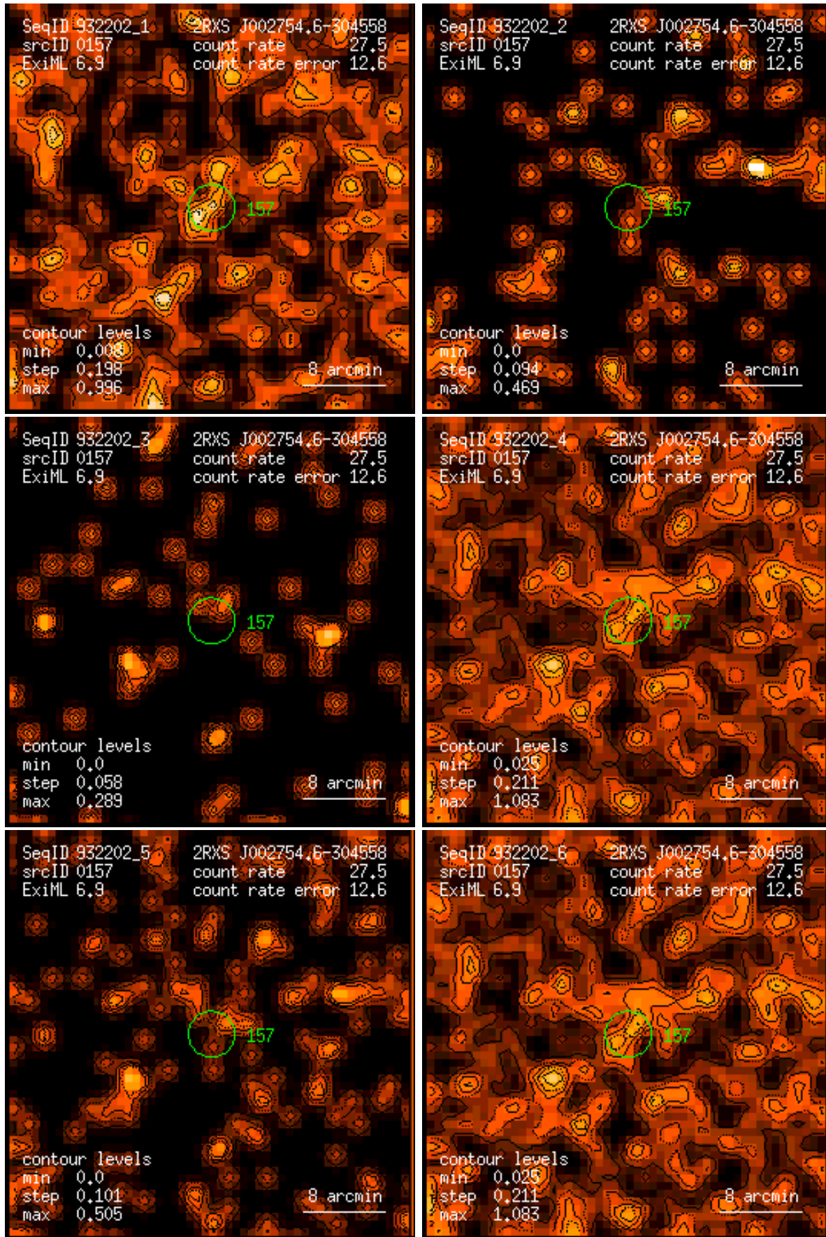
Figure 157: RASS 932202: detection 0157: band rate images, Gaussian filter: (1) PSPC channels 11 – 41, (2) 52 – 90, (3) 91 – 201, (4) 11 – 235, (5) 52 – 201, (6) 11 – 201. Broad band rates in counts/ks. Band rate contour levels in counts/ks/arcmin 2 .
