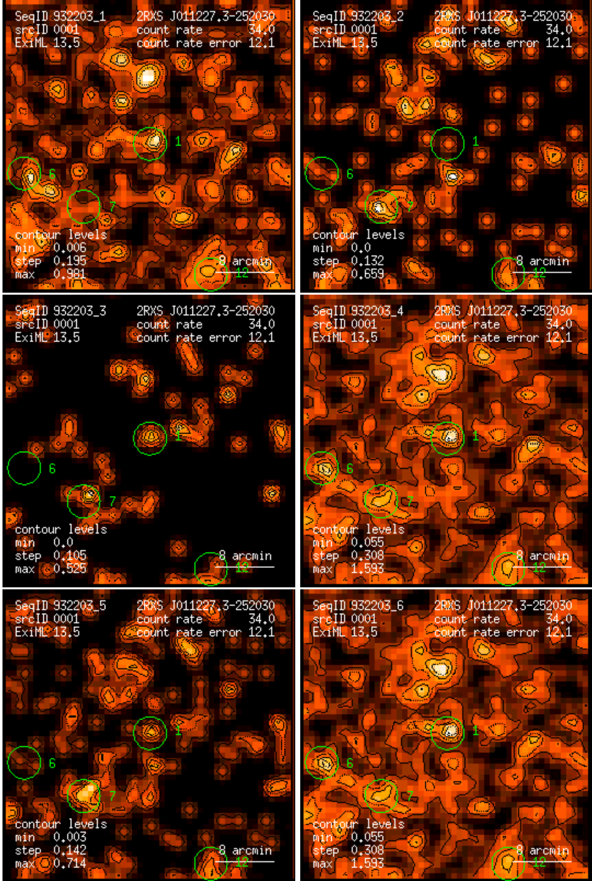
Figure 1: RASS 932203: detection 0001: band rate images, Gaussian filter: (1) PSPC channels 11 – 41, (2) 52 – 90, (3) 91 – 201, (4) 11 – 235, (5) 52 – 201, (6) 11 – 201. Broad band rates in counts/ks. Band rate contour levels in counts/ks/arcmin 2 .
