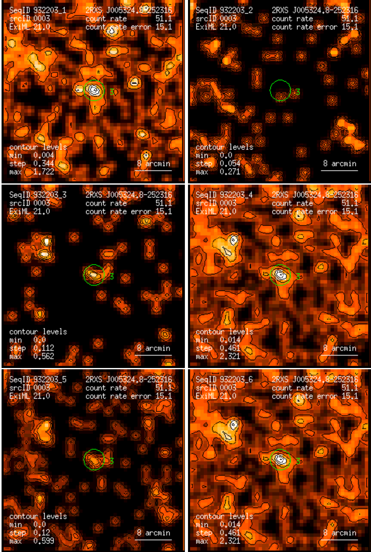
Figure 3: RASS 932203: detection 0003: band rate images, Gaussian filter: (1) PSPC channels 11 – 41, (2) 52 – 90, (3) 91 – 201, (4) 11 – 235, (5) 52 – 201, (6) 11 – 201. Broad band rates in counts/ks. Band rate contour levels in counts/ks/arcmin 2 .
