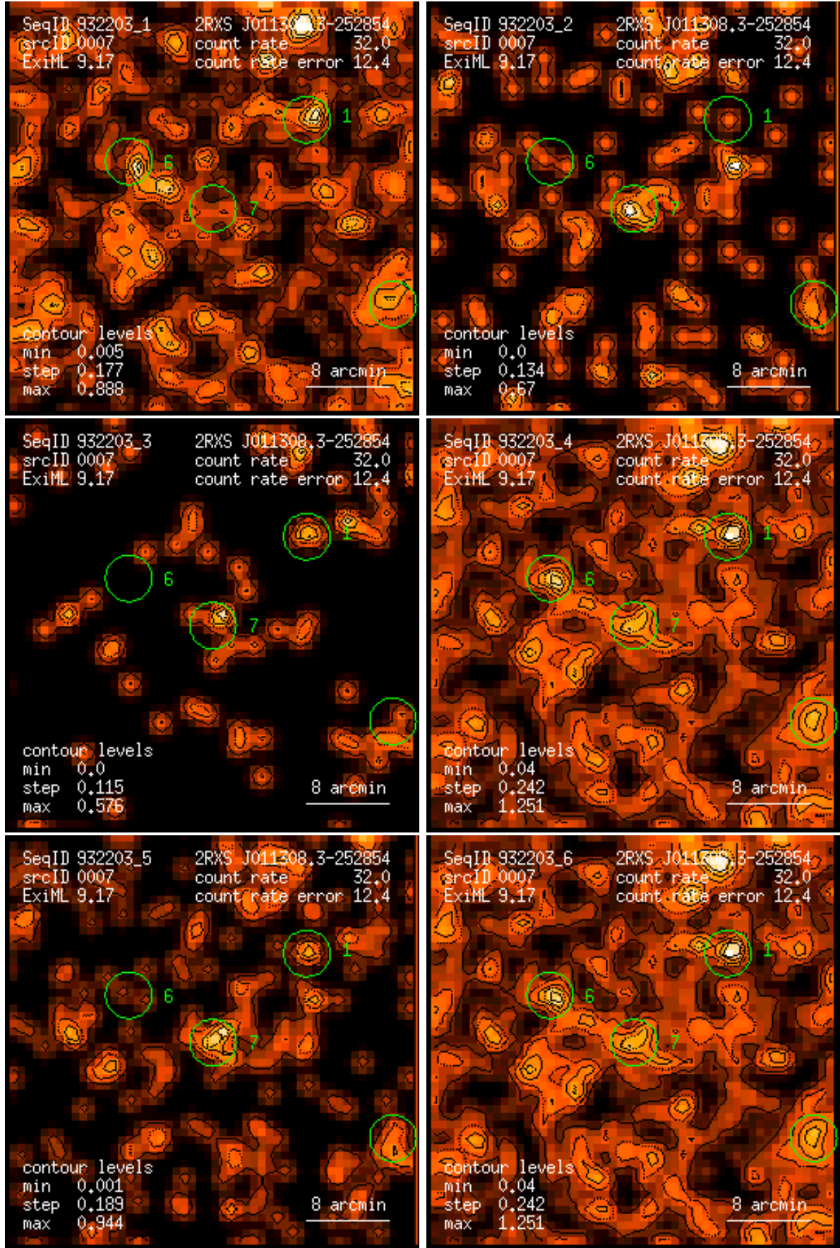
Figure 7: RASS 932203: detection 0007: band rate images, Gaussian filter: (1) PSPC channels 11 – 41, (2) 52 – 90, (3) 91 – 201, (4) 11 – 235, (5) 52 – 201, (6) 11 – 201. Broad band rates in counts/ks. Band rate contour levels in counts/ks/arcmin 2 .
