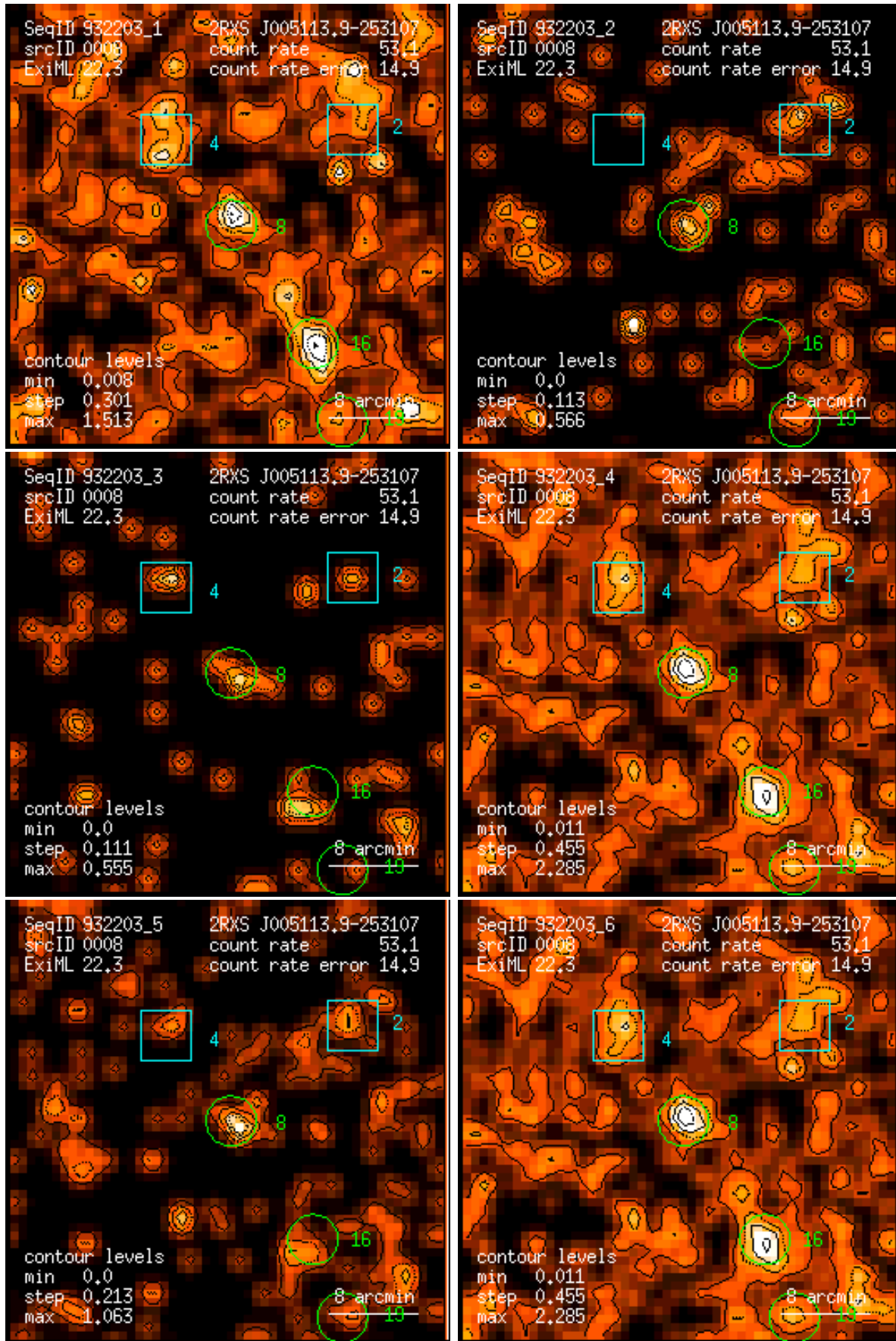
Figure 8: RASS 932203: detection 0008: band rate images, Gaussian filter: (1) PSPC channels 11 – 41, (2) 52 – 90, (3) 91 – 201, (4) 11 – 235, (5) 52 – 201, (6) 11 – 201. Broad band rates in counts/ks. Band rate contour levels in counts/ks/arcmin 2 .
