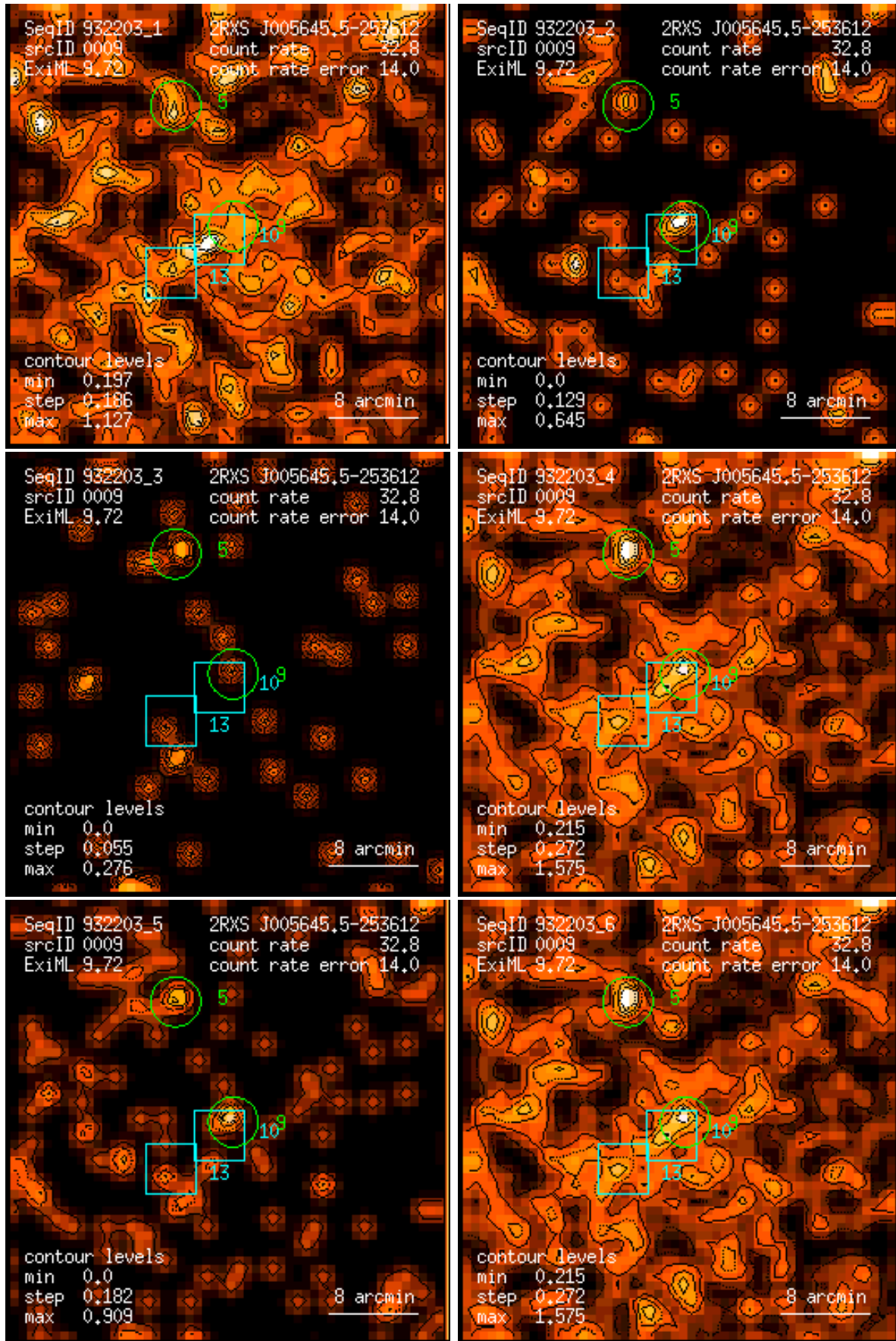
Figure 9: RASS 932203: detection 0009: band rate images, Gaussian filter: (1) PSPC channels 11 – 41, (2) 52 – 90, (3) 91 – 201, (4) 11 – 235, (5) 52 – 201, (6) 11 – 201. Broad band rates in counts/ks. Band rate contour levels in counts/ks/arcmin 2 .
