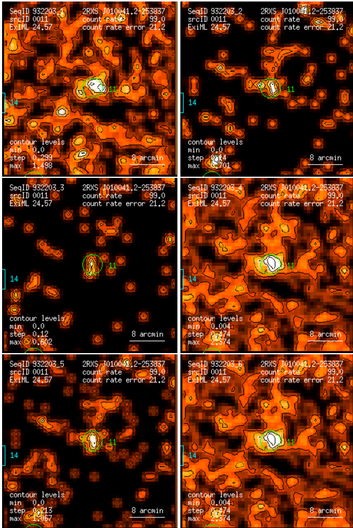
Figure 11: RASS 932203: detection 0011: band rate images, Gaussian filter: (1) PSPC channels 11 – 41, (2) 52 – 90, (3) 91 – 201, (4) 11 – 235, (5) 52 – 201, (6) 11 – 201. Broad band rates in counts/ks. Band rate contour levels in counts/ks/arcmin 2 .
