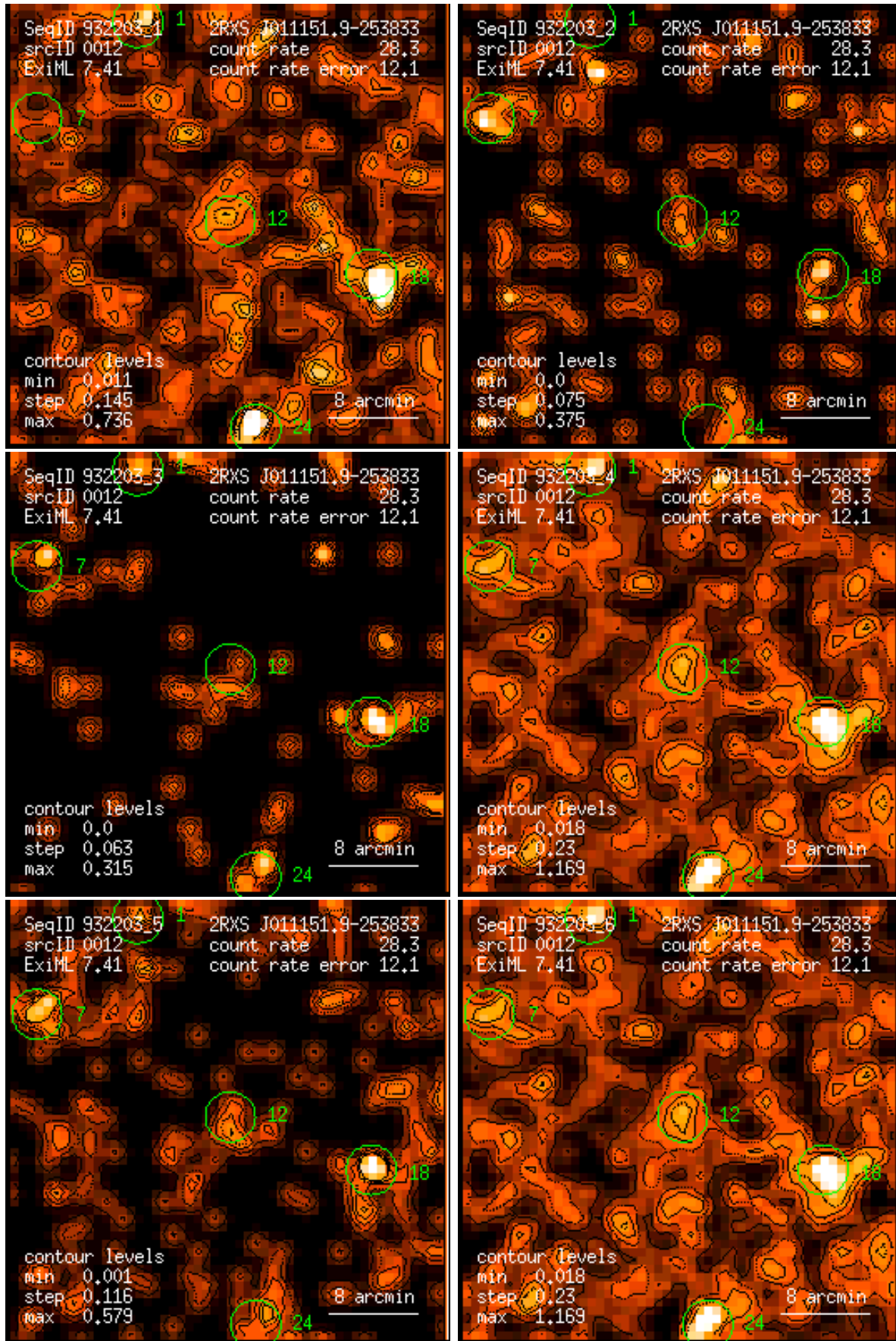
Figure 12: RASS 932203: detection 0012: band rate images, Gaussian filter: (1) PSPC channels 11 – 41, (2) 52 – 90, (3) 91 – 201, (4) 11 – 235, (5) 52 – 201, (6) 11 – 201. Broad band rates in counts/ks. Band rate contour levels in counts/ks/arcmin 2 .
