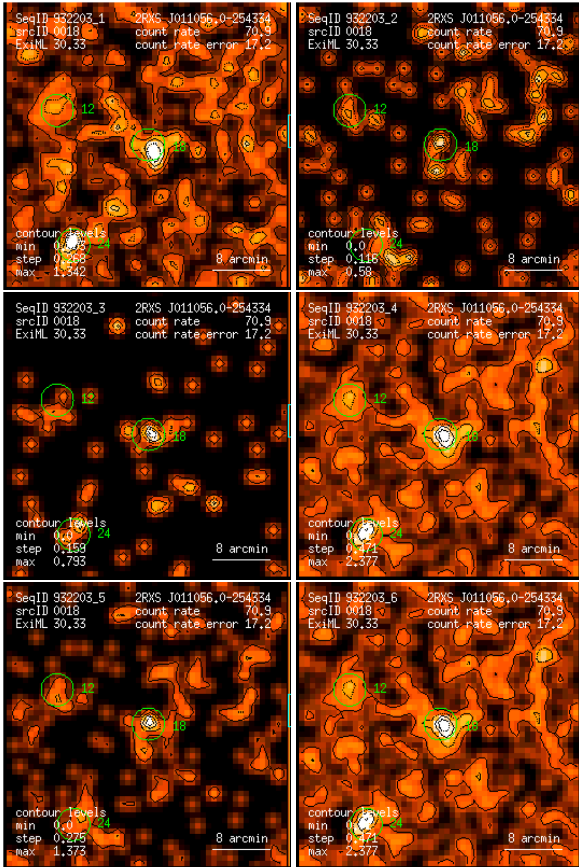
Figure 18: RASS 932203: detection 0018: band rate images, Gaussian filter: (1) PSPC channels 11 – 41, (2) 52 – 90, (3) 91 – 201, (4) 11 – 235, (5) 52 – 201, (6) 11 – 201. Broad band rates in counts/ks. Band rate contour levels in counts/ks/arcmin 2 .
