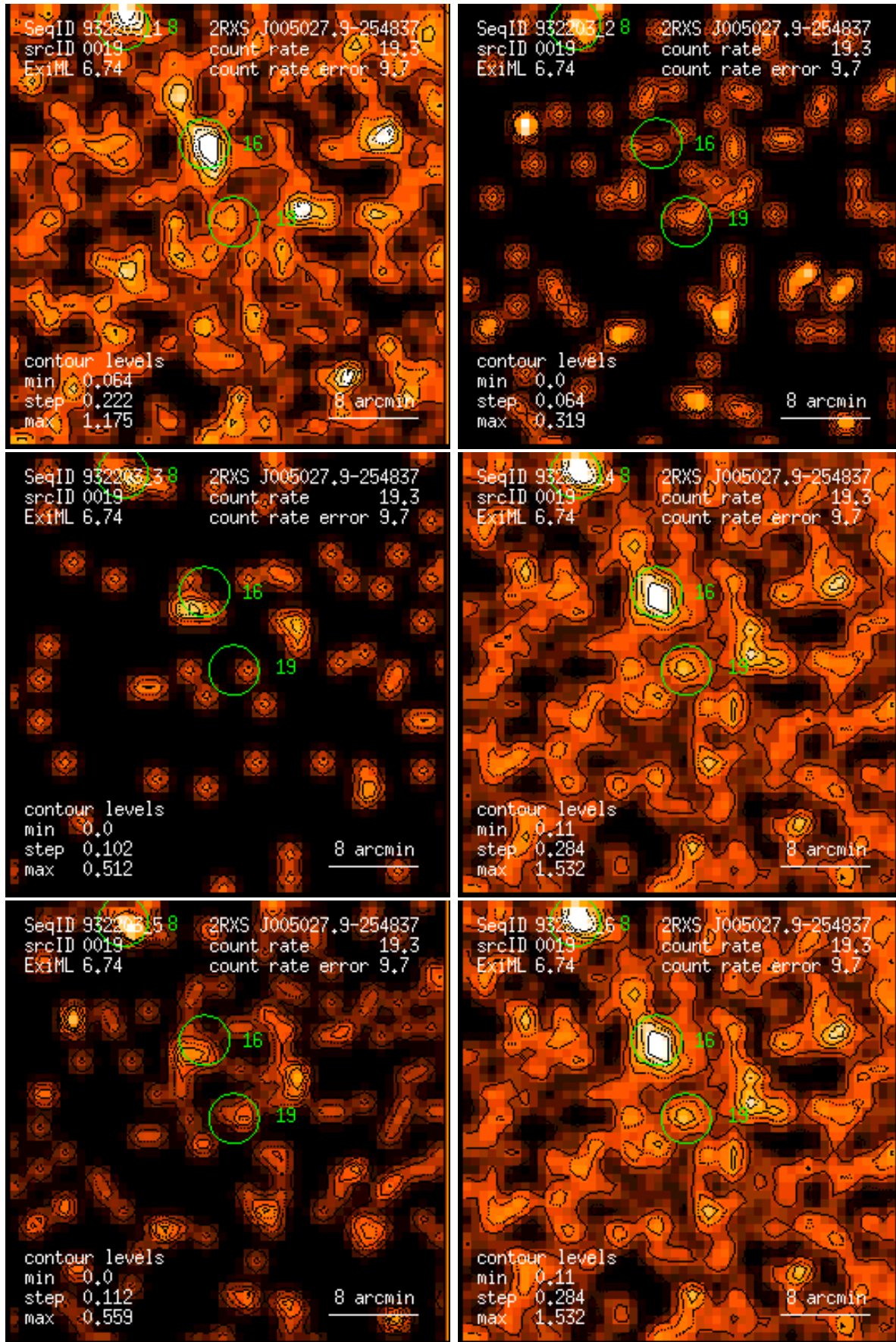
Figure 19: RASS 932203: detection 0019: band rate images, Gaussian filter: (1) PSPC channels 11 – 41, (2) 52 – 90, (3) 91 – 201, (4) 11 – 235, (5) 52 – 201, (6) 11 – 201. Broad band rates in counts/ks. Band rate contour levels in counts/ks/arcmin 2 .
