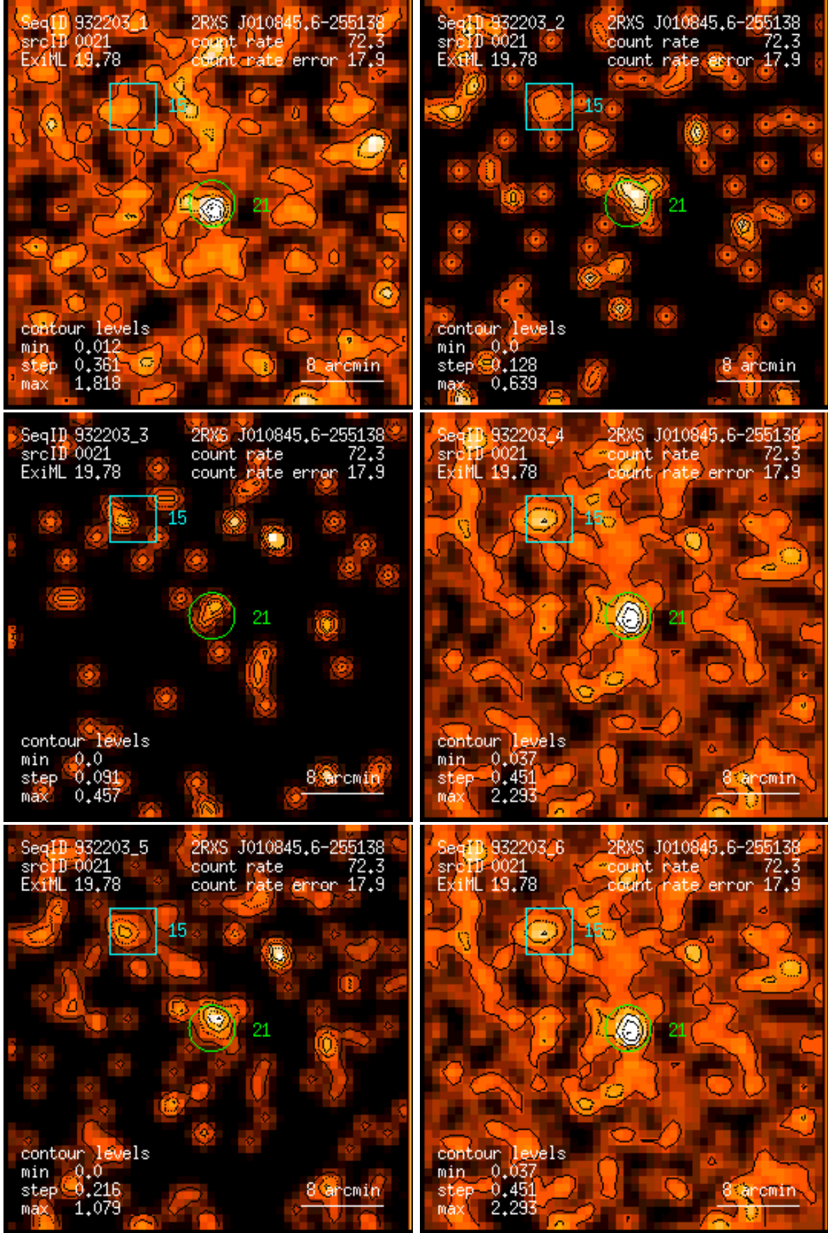
Figure 21: RASS 932203: detection 0021: band rate images, Gaussian filter: (1) PSPC channels 11 – 41, (2) 52 – 90, (3) 91 – 201, (4) 11 – 235, (5) 52 – 201, (6) 11 – 201. Broad band rates in counts/ks. Band rate contour levels in counts/ks/arcmin 2 .
