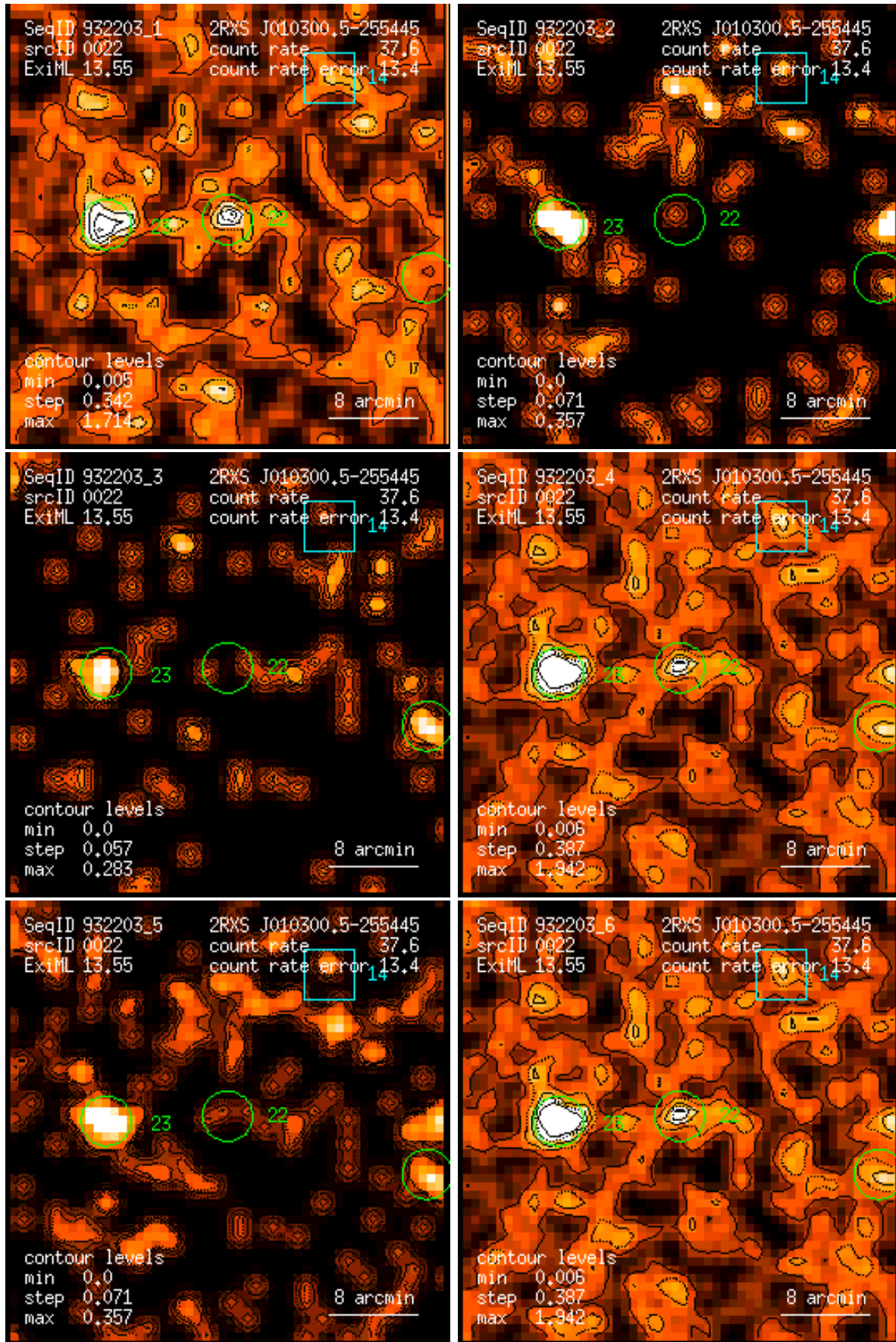
Figure 22: RASS 932203: detection 0022: band rate images, Gaussian filter: (1) PSPC channels 11 – 41, (2) 52 – 90, (3) 91 – 201, (4) 11 – 235, (5) 52 – 201, (6) 11 – 201. Broad band rates in counts/ks. Band rate contour levels in counts/ks/arcmin 2 .
