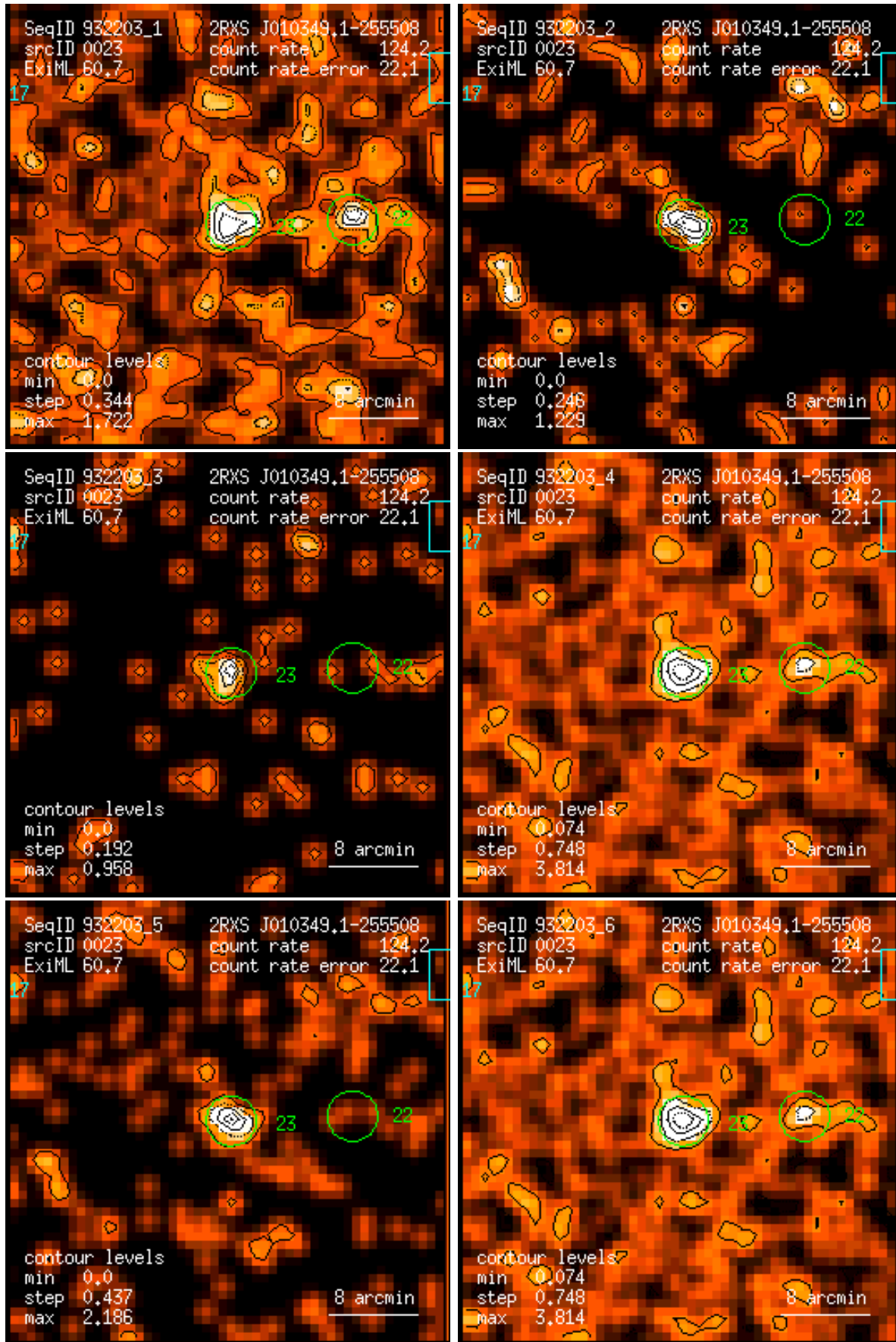
Figure 23: RASS 932203: detection 0023: band rate images, Gaussian filter: (1) PSPC channels 11 – 41, (2) 52 – 90, (3) 91 – 201, (4) 11 – 235, (5) 52 – 201, (6) 11 – 201. Broad band rates in counts/ks. Band rate contour levels in counts/ks/arcmin 2 .
