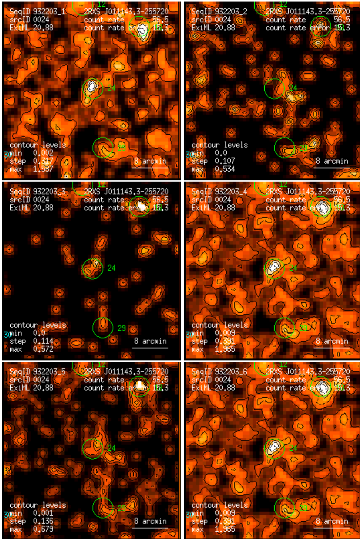
Figure 24: RASS 932203: detection 0024: band rate images, Gaussian filter: (1) PSPC channels 11 – 41, (2) 52 – 90, (3) 91 – 201, (4) 11 – 235, (5) 52 – 201, (6) 11 – 201. Broad band rates in counts/ks. Band rate contour levels in counts/ks/arcmin 2 .
