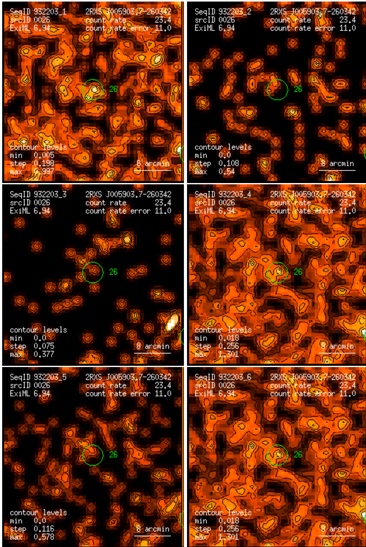
Figure 26: RASS 932203: detection 0026: band rate images, Gaussian filter: (1) PSPC channels 11 – 41, (2) 52 – 90, (3) 91 – 201, (4) 11 – 235, (5) 52 – 201, (6) 11 – 201. Broad band rates in counts/ks. Band rate contour levels in counts/ks/arcmin 2 .
