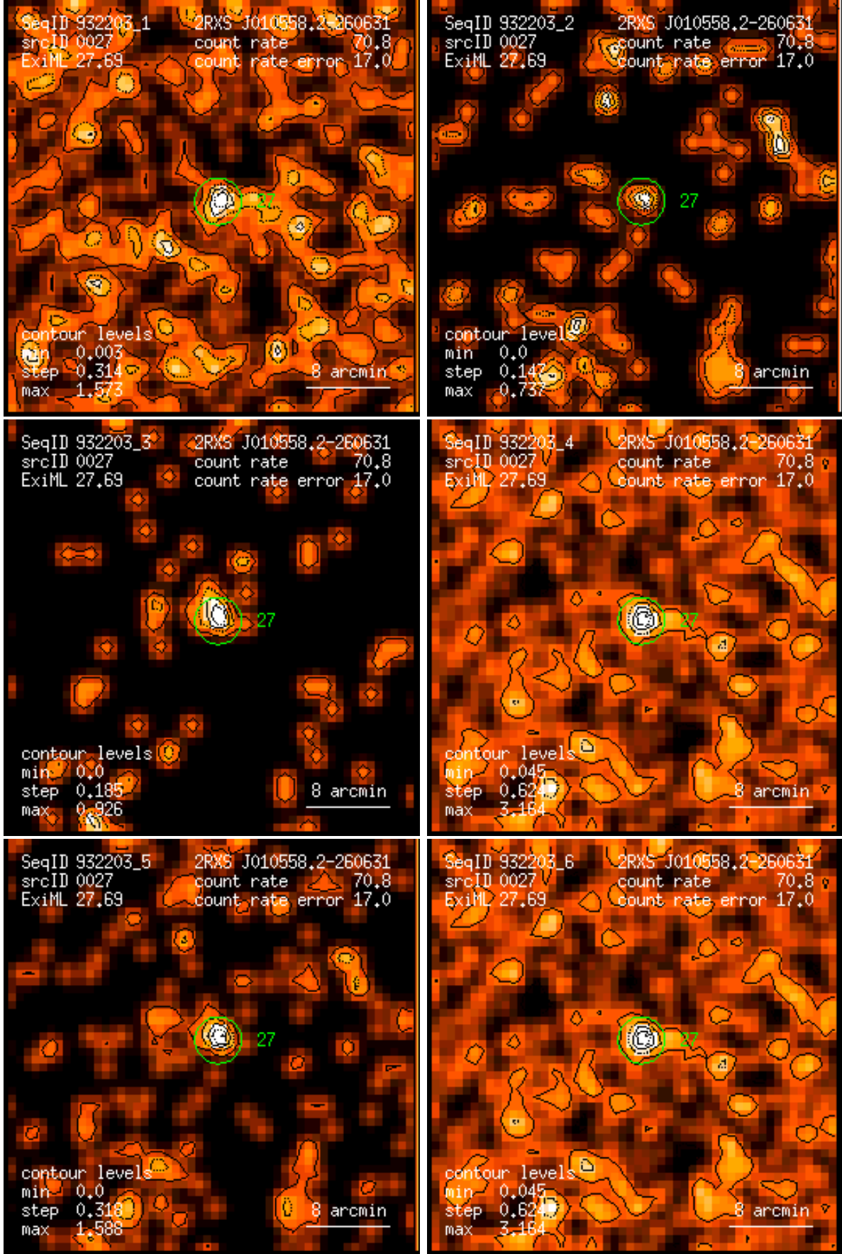
Figure 27: RASS 932203: detection 0027: band rate images, Gaussian filter: (1) PSPC channels 11 – 41, (2) 52 – 90, (3) 91 – 201, (4) 11 – 235, (5) 52 – 201, (6) 11 – 201. Broad band rates in counts/ks. Band rate contour levels in counts/ks/arcmin 2 .
