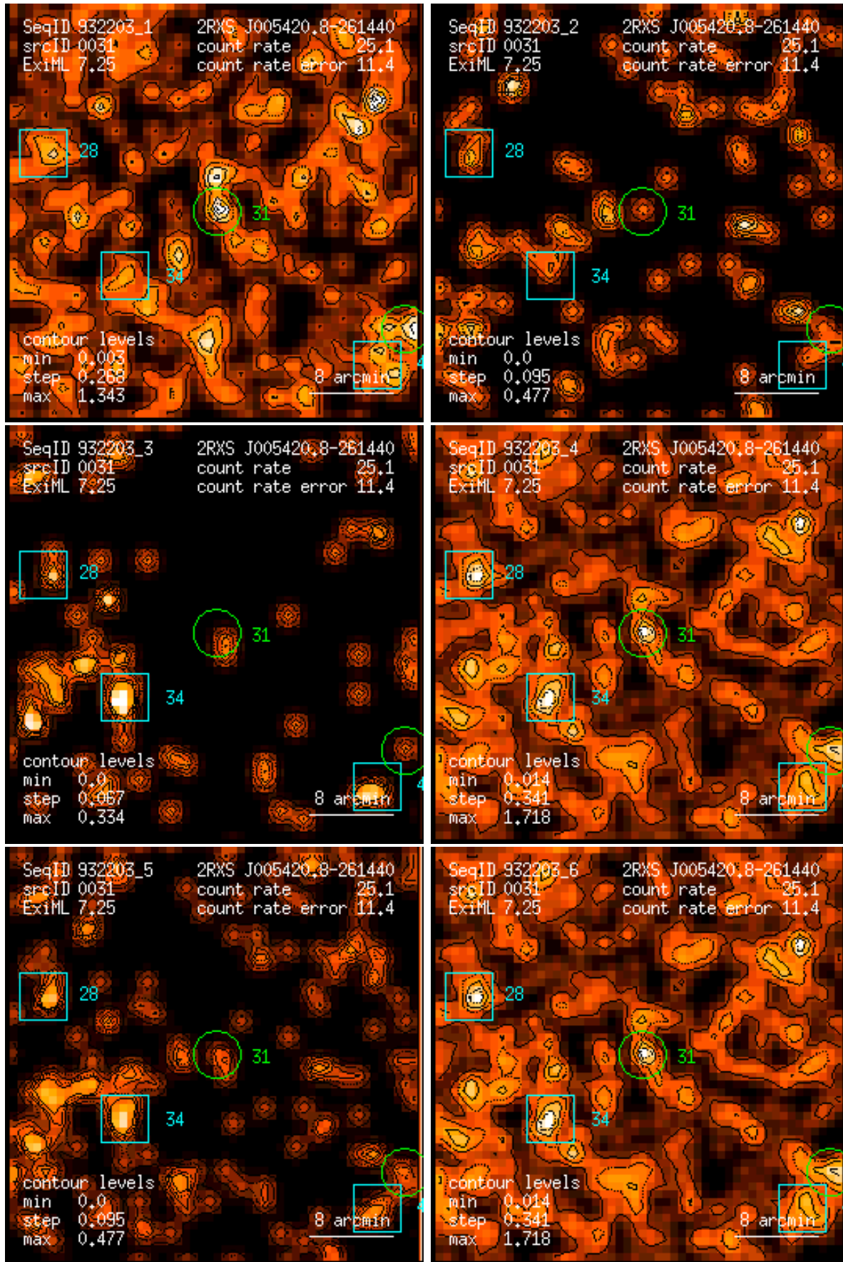
Figure 31: RASS 932203: detection 0031: band rate images, Gaussian filter: (1) PSPC channels 11 – 41, (2) 52 – 90, (3) 91 – 201, (4) 11 – 235, (5) 52 – 201, (6) 11 – 201. Broad band rates in counts/ks. Band rate contour levels in counts/ks/arcmin 2 .
