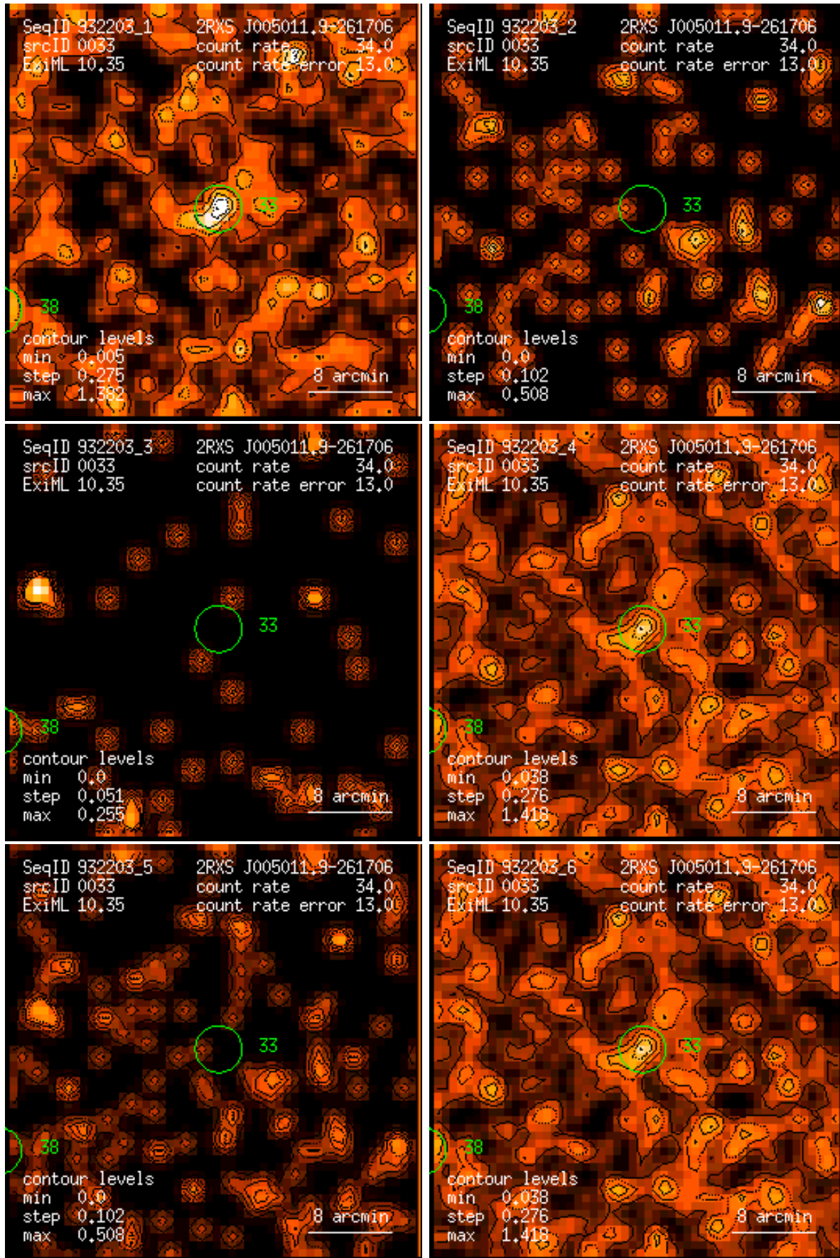
Figure 33: RASS 932203: detection 0033: band rate images, Gaussian filter: (1) PSPC channels 11 – 41, (2) 52 – 90, (3) 91 – 201, (4) 11 – 235, (5) 52 – 201, (6) 11 – 201. Broad band rates in counts/ks. Band rate contour levels in counts/ks/arcmin 2 .
