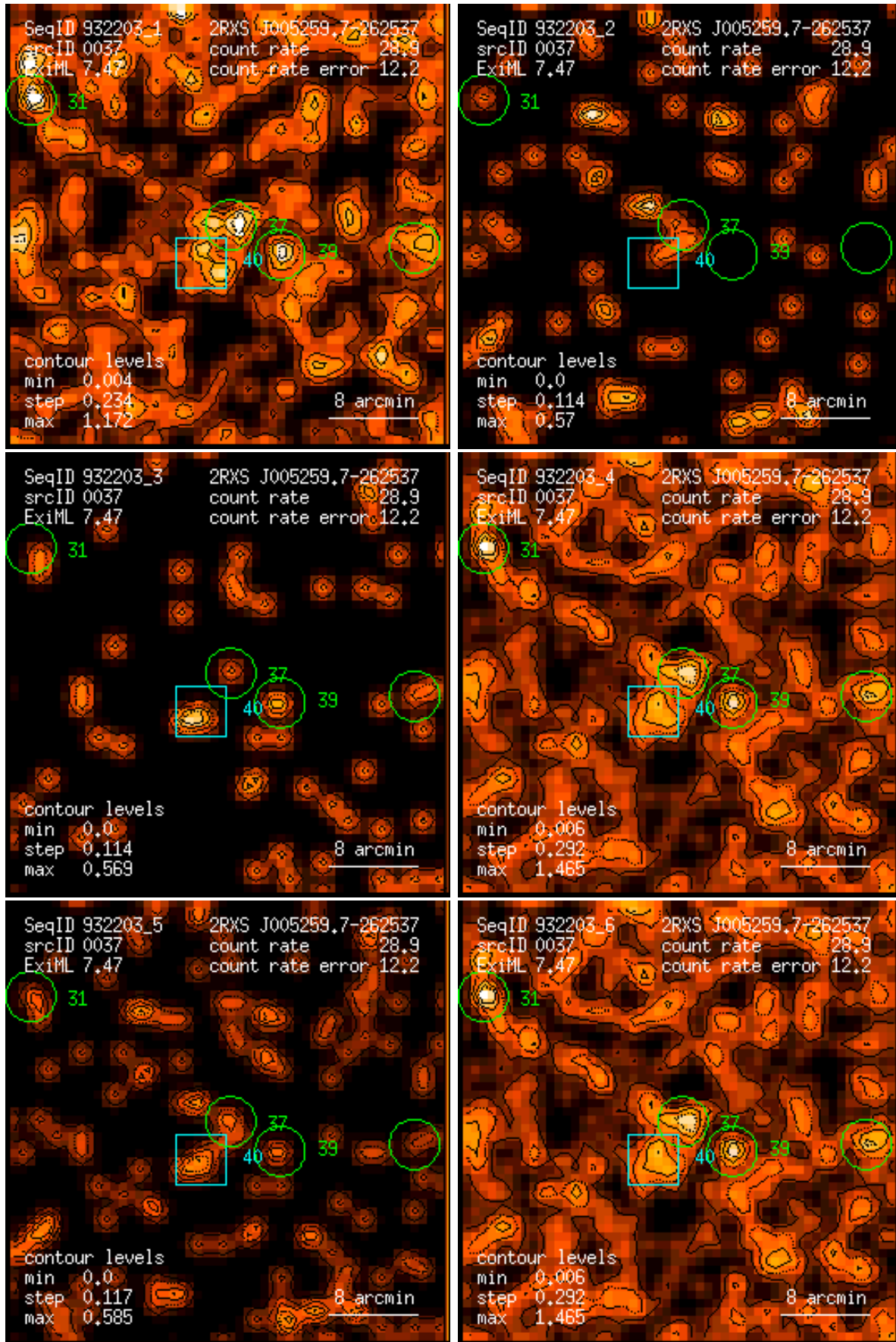
Figure 37: RASS 932203: detection 0037: band rate images, Gaussian filter: (1) PSPC channels 11 – 41, (2) 52 – 90, (3) 91 – 201, (4) 11 – 235, (5) 52 – 201, (6) 11 – 201. Broad band rates in counts/ks. Band rate contour levels in counts/ks/arcmin 2 .
