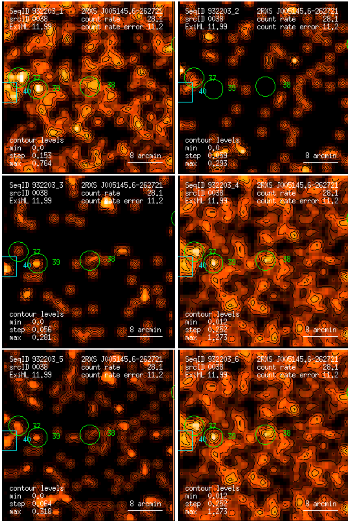
Figure 38: RASS 932203: detection 0038: band rate images, Gaussian filter: (1) PSPC channels 11 – 41, (2) 52 – 90, (3) 91 – 201, (4) 11 – 235, (5) 52 – 201, (6) 11 – 201. Broad band rates in counts/ks. Band rate contour levels in counts/ks/arcmin 2 .
