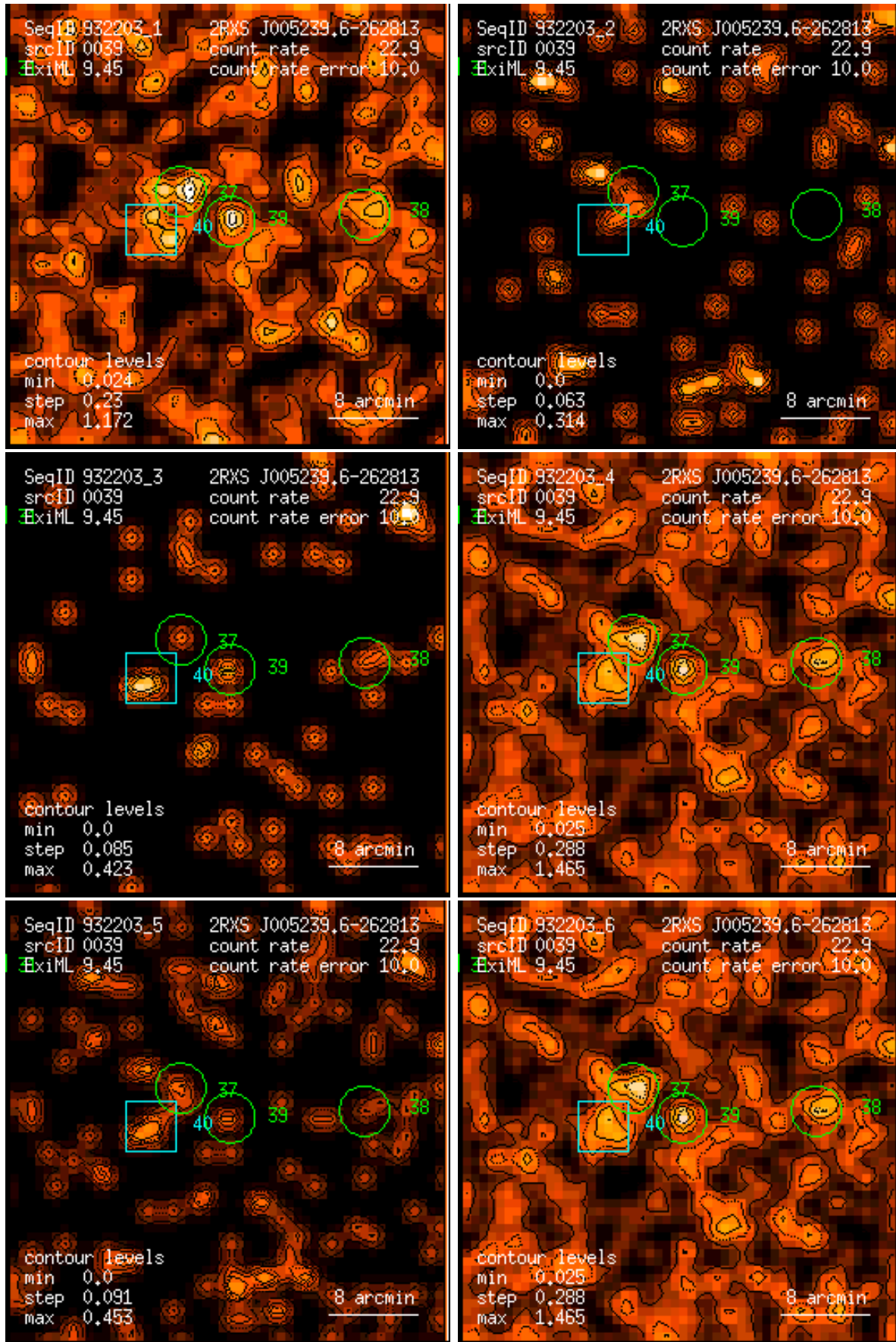
Figure 39: RASS 932203: detection 0039: band rate images, Gaussian filter: (1) PSPC channels 11 – 41, (2) 52 – 90, (3) 91 – 201, (4) 11 – 235, (5) 52 – 201, (6) 11 – 201. Broad band rates in counts/ks. Band rate contour levels in counts/ks/arcmin 2 .
