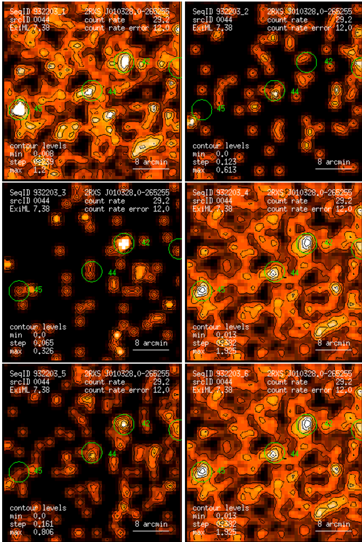
Figure 44: RASS 932203: detection 0044: band rate images, Gaussian filter: (1) PSPC channels 11 – 41, (2) 52 – 90, (3) 91 – 201, (4) 11 – 235, (5) 52 – 201, (6) 11 – 201. Broad band rates in counts/ks. Band rate contour levels in counts/ks/arcmin 2 .
