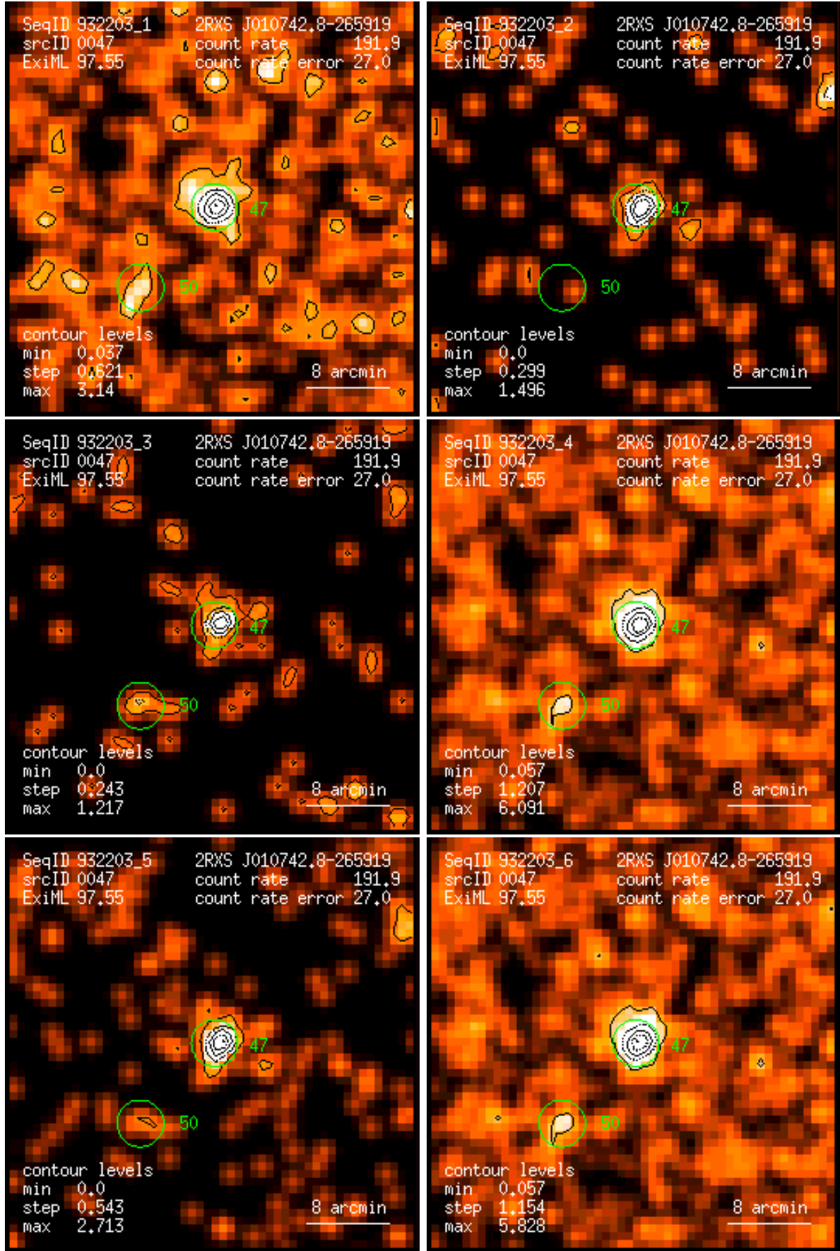
Figure 47: RASS 932203: detection 0047: band rate images, Gaussian filter: (1) PSPC channels 11 – 41, (2) 52 – 90, (3) 91 – 201, (4) 11 – 235, (5) 52 – 201, (6) 11 – 201. Broad band rates in counts/ks. Band rate contour levels in counts/ks/arcmin 2 .
