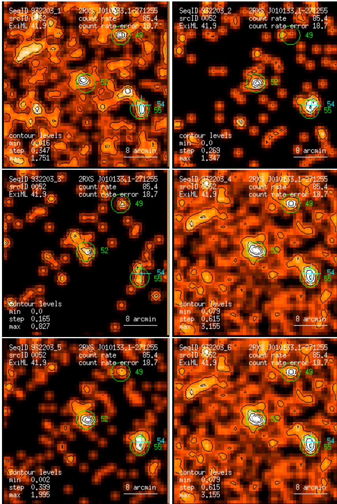
Figure 52: RASS 932203: detection 0052: band rate images, Gaussian filter: (1) PSPC channels 11 – 41, (2) 52 – 90, (3) 91 – 201, (4) 11 – 235, (5) 52 – 201, (6) 11 – 201. Broad band rates in counts/ks. Band rate contour levels in counts/ks/arcmin 2 .
