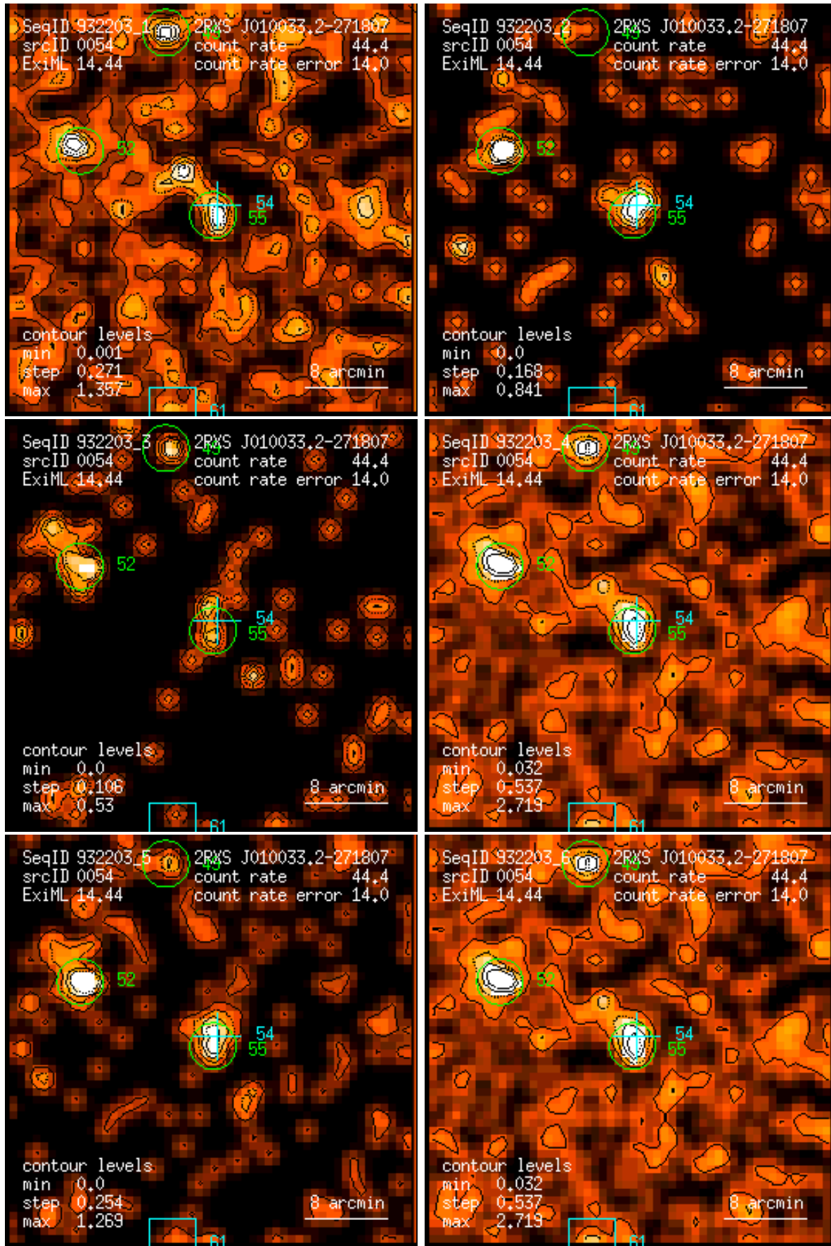
Figure 54: RASS 932203: detection 0054: band rate images, Gaussian filter: (1) PSPC channels 11 – 41, (2) 52 – 90, (3) 91 – 201, (4) 11 – 235, (5) 52 – 201, (6) 11 – 201. Broad band rates in counts/ks. Band rate contour levels in counts/ks/arcmin 2 .
