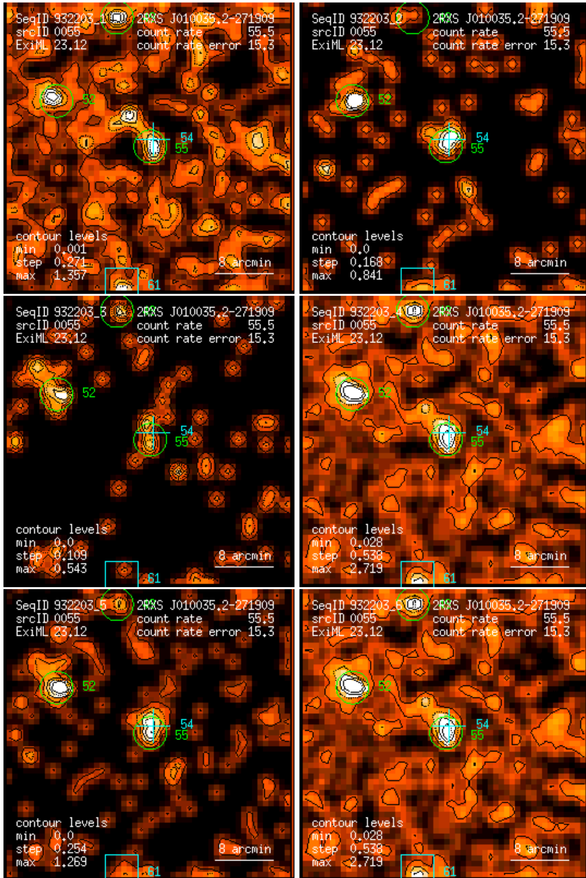
Figure 55: RASS 932203: detection 0055: band rate images, Gaussian filter: (1) PSPC channels 11 – 41, (2) 52 – 90, (3) 91 – 201, (4) 11 – 235, (5) 52 – 201, (6) 11 – 201. Broad band rates in counts/ks. Band rate contour levels in counts/ks/arcmin 2 .
