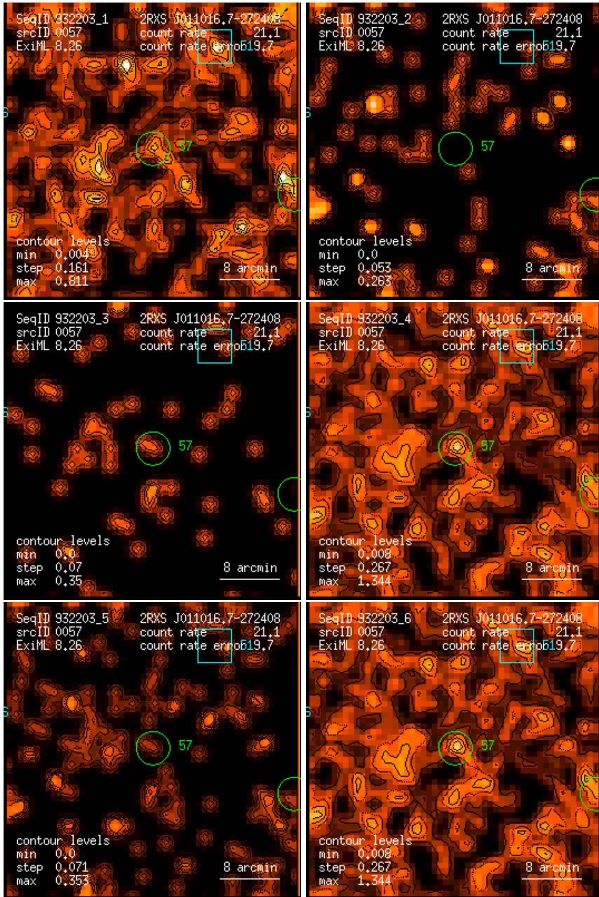
Figure 57: RASS 932203: detection 0057: band rate images, Gaussian filter: (1) PSPC channels 11 – 41, (2) 52 – 90, (3) 91 – 201, (4) 11 – 235, (5) 52 – 201, (6) 11 – 201. Broad band rates in counts/ks. Band rate contour levels in counts/ks/arcmin 2 .
