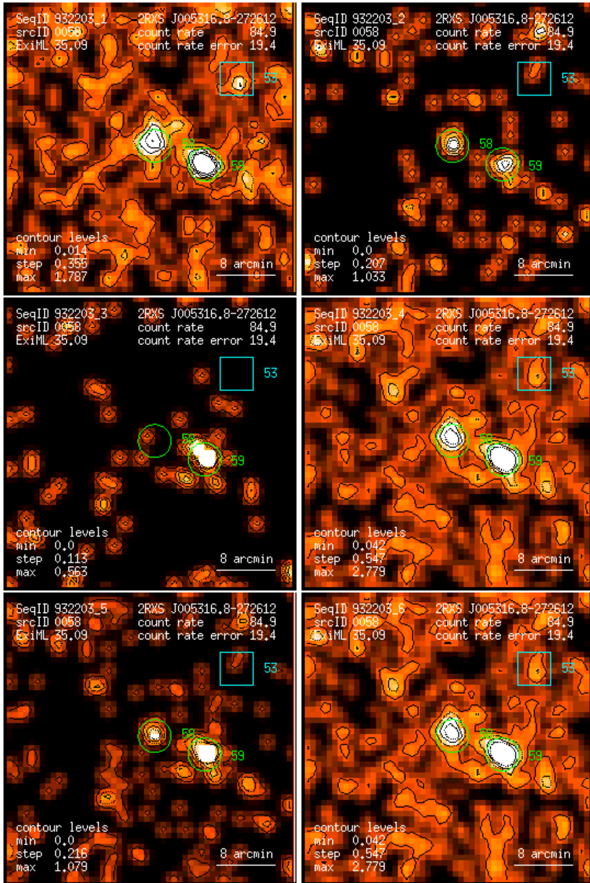
Figure 58: RASS 932203: detection 0058: band rate images, Gaussian filter: (1) PSPC channels 11 – 41, (2) 52 – 90, (3) 91 – 201, (4) 11 – 235, (5) 52 – 201, (6) 11 – 201. Broad band rates in counts/ks. Band rate contour levels in counts/ks/arcmin 2 .
