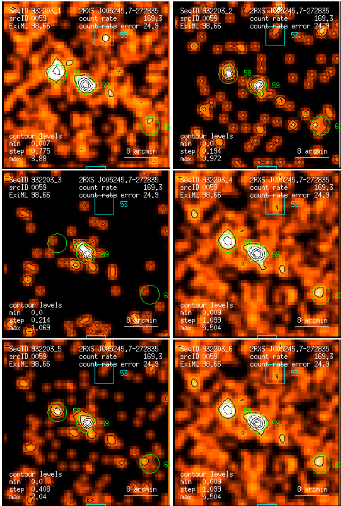
Figure 59: RASS 932203: detection 0059: band rate images, Gaussian filter: (1) PSPC channels 11 – 41, (2) 52 – 90, (3) 91 – 201, (4) 11 – 235, (5) 52 – 201, (6) 11 – 201. Broad band rates in counts/ks. Band rate contour levels in counts/ks/arcmin 2 .
