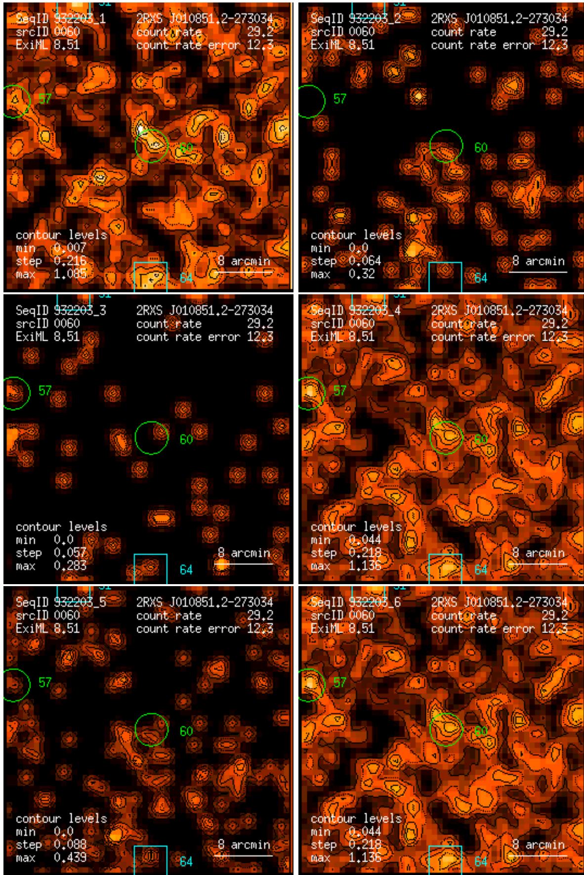
Figure 60: RASS 932203: detection 0060: band rate images, Gaussian filter: (1) PSPC channels 11 – 41, (2) 52 – 90, (3) 91 – 201, (4) 11 – 235, (5) 52 – 201, (6) 11 – 201. Broad band rates in counts/ks. Band rate contour levels in counts/ks/arcmin 2 .
