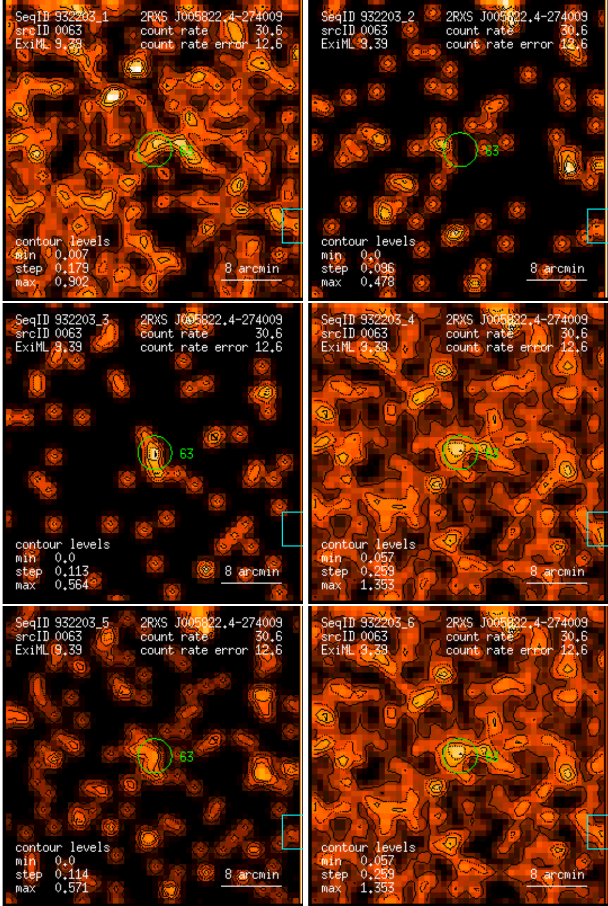
Figure 63: RASS 932203: detection 0063: band rate images, Gaussian filter: (1) PSPC channels 11 – 41, (2) 52 – 90, (3) 91 – 201, (4) 11 – 235, (5) 52 – 201, (6) 11 – 201. Broad band rates in counts/ks. Band rate contour levels in counts/ks/arcmin 2 .
