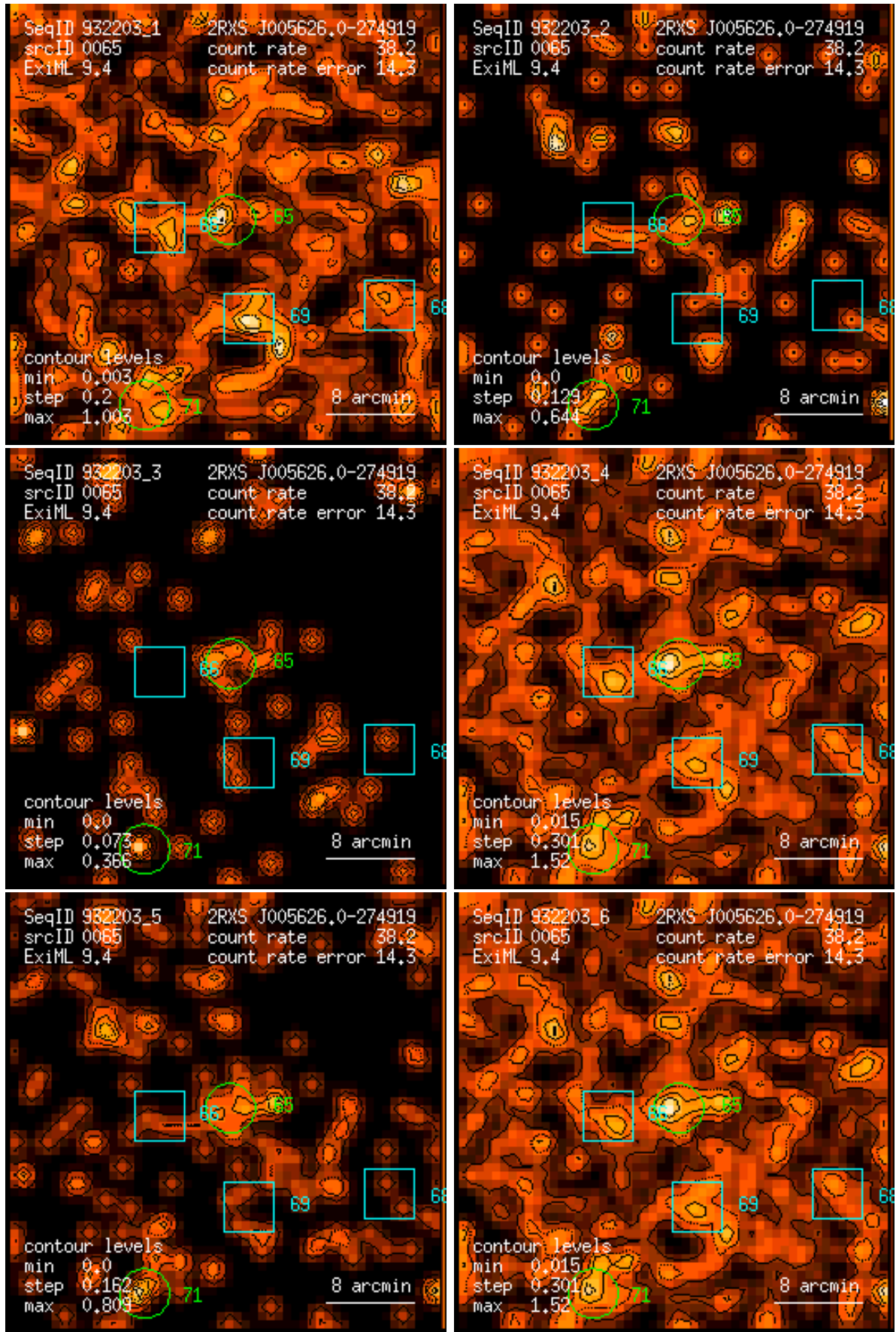
Figure 65: RASS 932203: detection 0065: band rate images, Gaussian filter: (1) PSPC channels 11 – 41, (2) 52 – 90, (3) 91 – 201, (4) 11 – 235, (5) 52 – 201, (6) 11 – 201. Broad band rates in counts/ks. Band rate contour levels in counts/ks/arcmin 2 .
