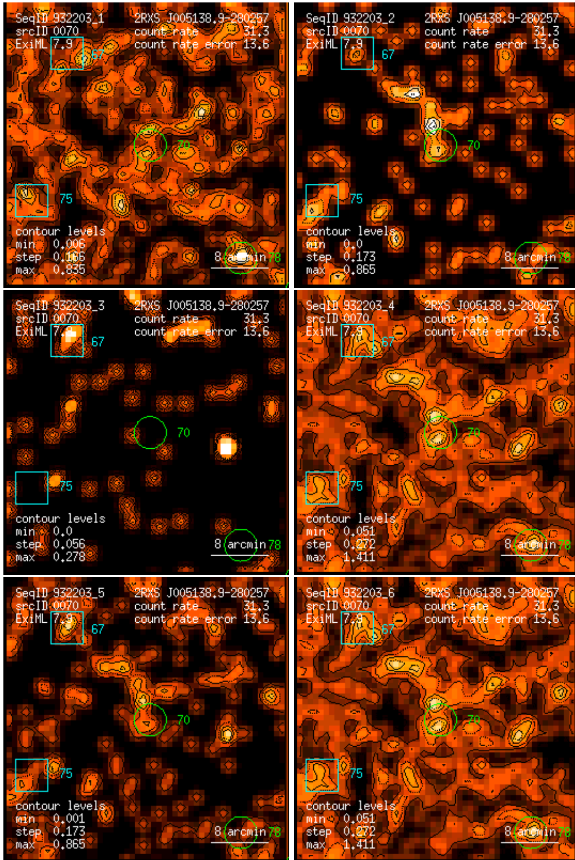
Figure 70: RASS 932203: detection 0070: band rate images, Gaussian filter: (1) PSPC channels 11 – 41, (2) 52 – 90, (3) 91 – 201, (4) 11 – 235, (5) 52 – 201, (6) 11 – 201. Broad band rates in counts/ks. Band rate contour levels in counts/ks/arcmin 2 .
