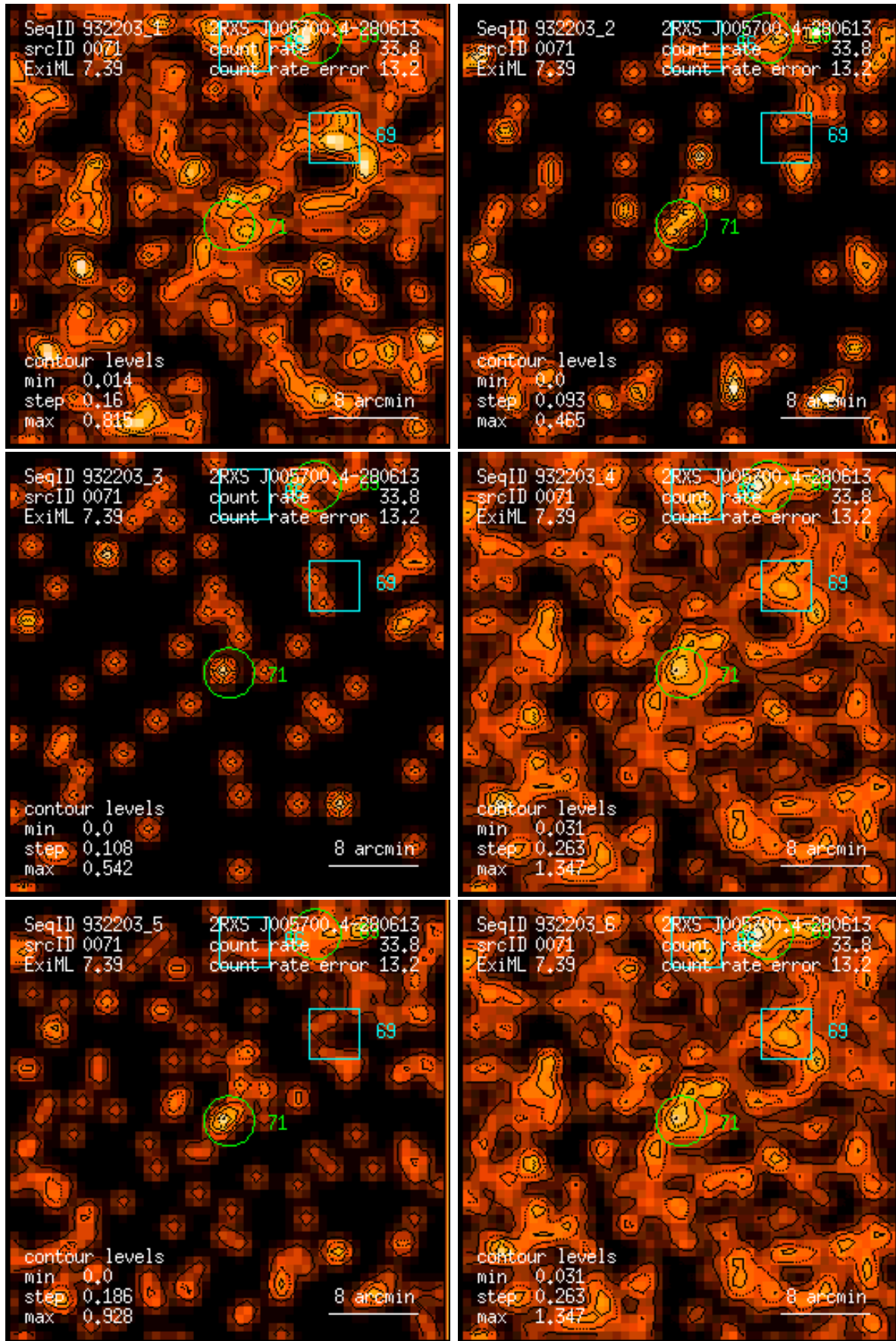
Figure 71: RASS 932203: detection 0071: band rate images, Gaussian filter: (1) PSPC channels 11 – 41, (2) 52 – 90, (3) 91 – 201, (4) 11 – 235, (5) 52 – 201, (6) 11 – 201. Broad band rates in counts/ks. Band rate contour levels in counts/ks/arcmin 2 .
